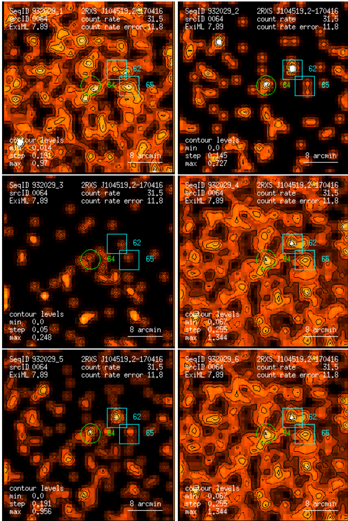
Figure 64: RASS 932029: detection 0064: band rate images, Gaussian filter: (1) PSPC channels 11 – 41, (2) 52 – 90, (3) 91 – 201, (4) 11 – 235, (5) 52 – 201, (6) 11 – 201. Broad band rates in counts/ks. Band rate contour levels in counts/ks/arcmin 2 .
