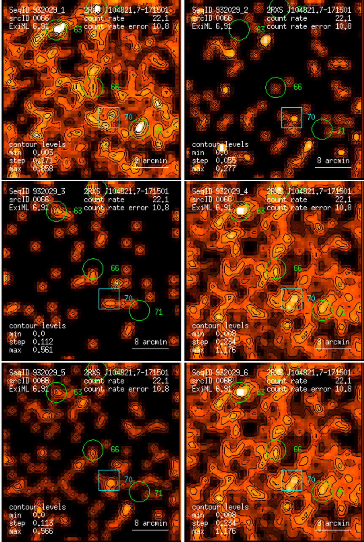
Figure 66: RASS 932029: detection 0066: band rate images, Gaussian filter: (1) PSPC channels 11 – 41, (2) 52 – 90, (3) 91 – 201, (4) 11 – 235, (5) 52 – 201, (6) 11 – 201. Broad band rates in counts/ks. Band rate contour levels in counts/ks/arcmin 2 .
