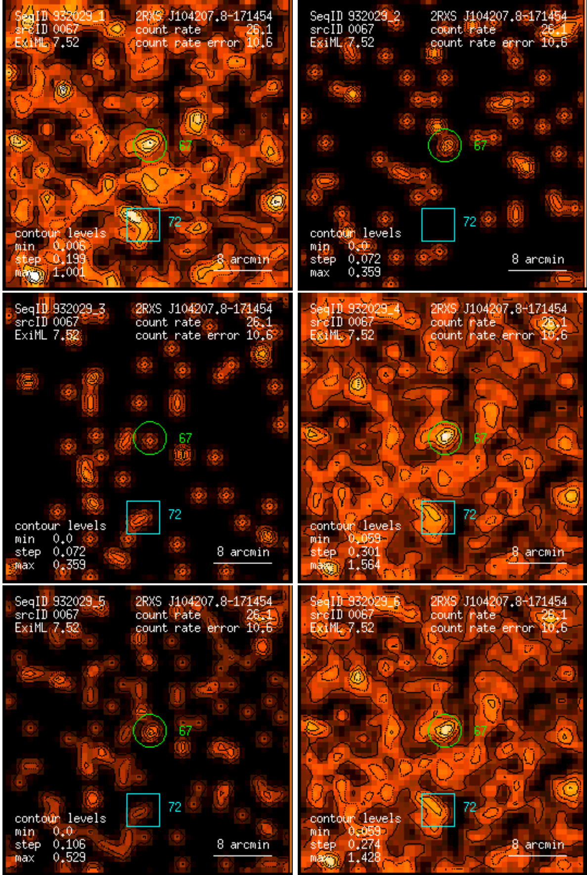
Figure 67: RASS 932029: detection 0067: band rate images, Gaussian filter: (1) PSPC channels 11 – 41, (2) 52 – 90, (3) 91 – 201, (4) 11 – 235, (5) 52 – 201, (6) 11 – 201. Broad band rates in counts/ks. Band rate contour levels in counts/ks/arcmin 2 .
