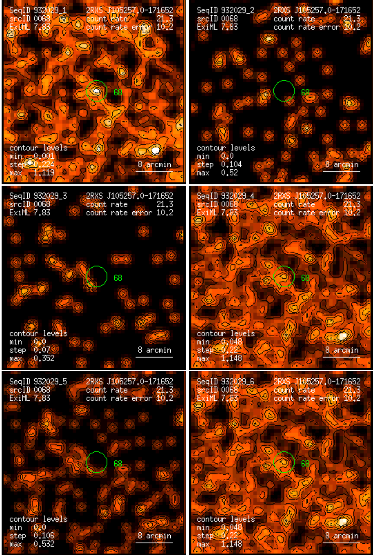
Figure 68: RASS 932029: detection 0068: band rate images, Gaussian filter: (1) PSPC channels 11 – 41, (2) 52 – 90, (3) 91 – 201, (4) 11 – 235, (5) 52 – 201, (6) 11 – 201. Broad band rates in counts/ks. Band rate contour levels in counts/ks/arcmin 2 .
