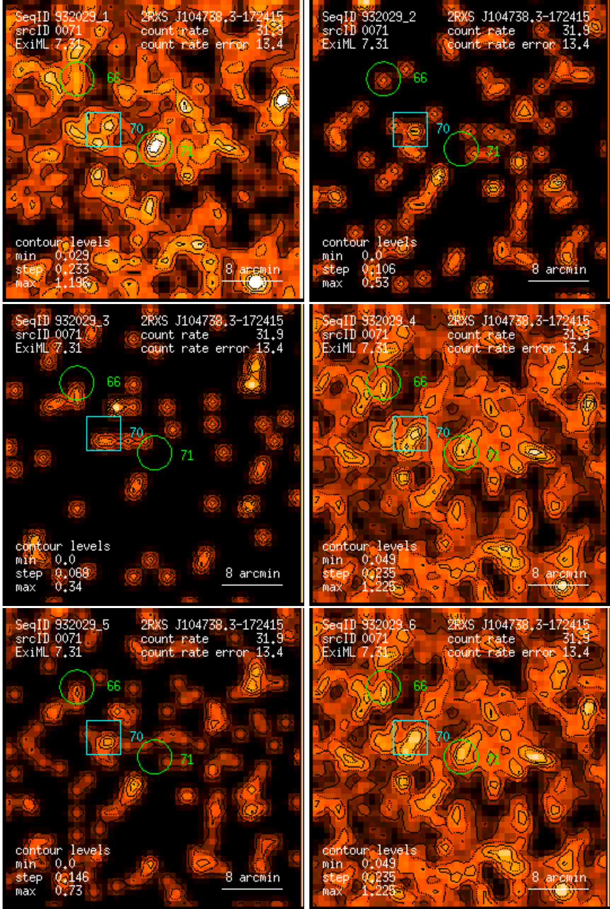
Figure 71: RASS 932029: detection 0071: band rate images, Gaussian filter: (1) PSPC channels 11 – 41, (2) 52 – 90, (3) 91 – 201, (4) 11 – 235, (5) 52 – 201, (6) 11 – 201. Broad band rates in counts/ks. Band rate contour levels in counts/ks/arcmin 2 .
