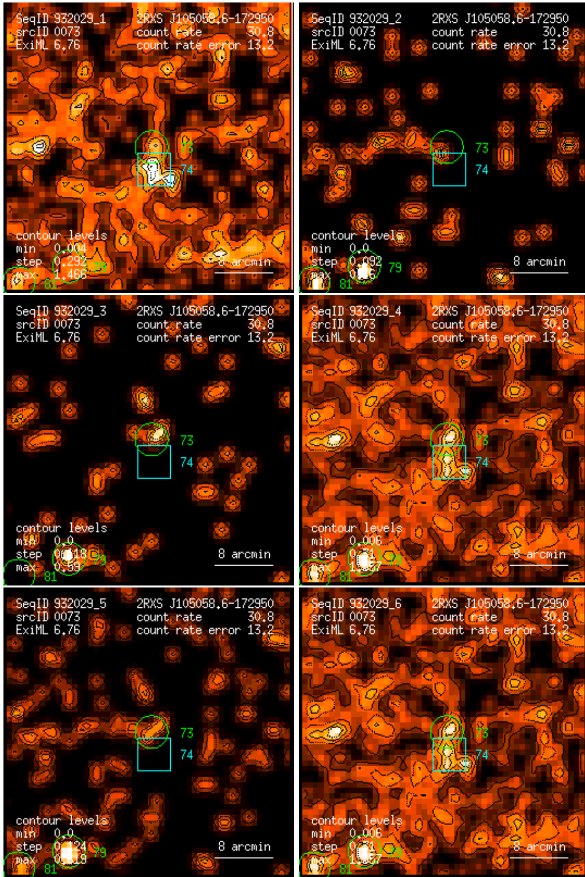
Figure 73: RASS 932029: detection 0073: band rate images, Gaussian filter: (1) PSPC channels 11 – 41, (2) 52 – 90, (3) 91 – 201, (4) 11 – 235, (5) 52 – 201, (6) 11 – 201. Broad band rates in counts/ks. Band rate contour levels in counts/ks/arcmin 2 .
