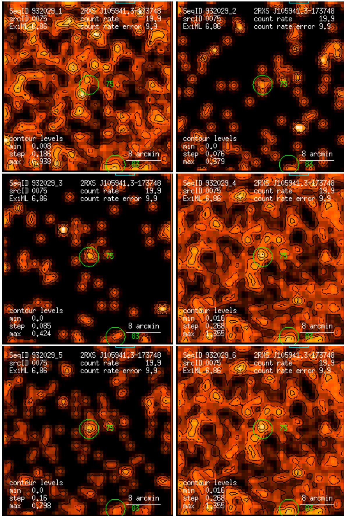
Figure 75: RASS 932029: detection 0075: band rate images, Gaussian filter: (1) PSPC channels 11 – 41, (2) 52 – 90, (3) 91 – 201, (4) 11 – 235, (5) 52 – 201, (6) 11 – 201. Broad band rates in counts/ks. Band rate contour levels in counts/ks/arcmin 2 .
