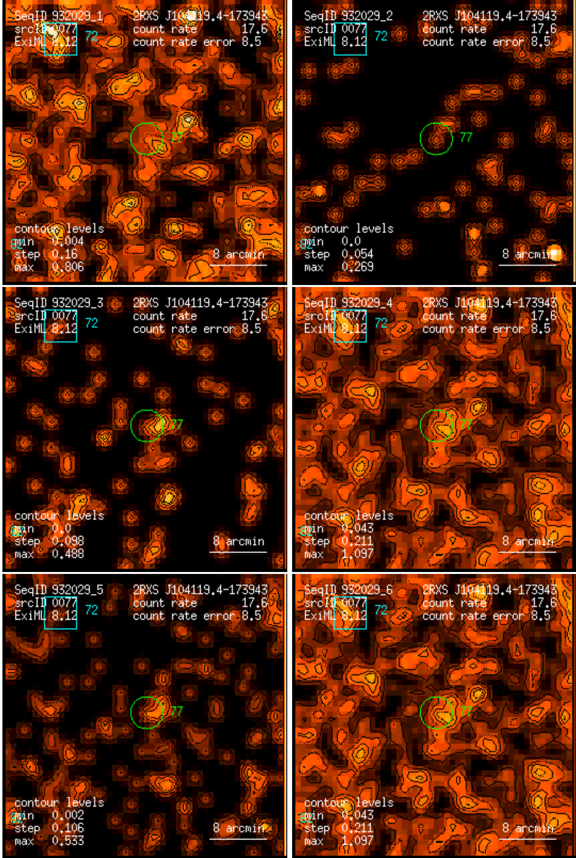
Figure 77: RASS 932029: detection 0077: band rate images, Gaussian filter: (1) PSPC channels 11 – 41, (2) 52 – 90, (3) 91 – 201, (4) 11 – 235, (5) 52 – 201, (6) 11 – 201. Broad band rates in counts/ks. Band rate contour levels in counts/ks/arcmin 2 .
