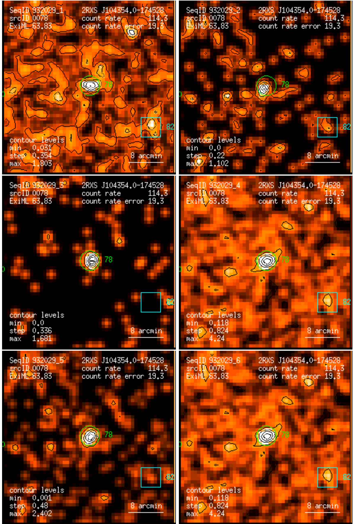
Figure 78: RASS 932029: detection 0078: band rate images, Gaussian filter: (1) PSPC channels 11 – 41, (2) 52 – 90, (3) 91 – 201, (4) 11 – 235, (5) 52 – 201, (6) 11 – 201. Broad band rates in counts/ks. Band rate contour levels in counts/ks/arcmin 2 .
