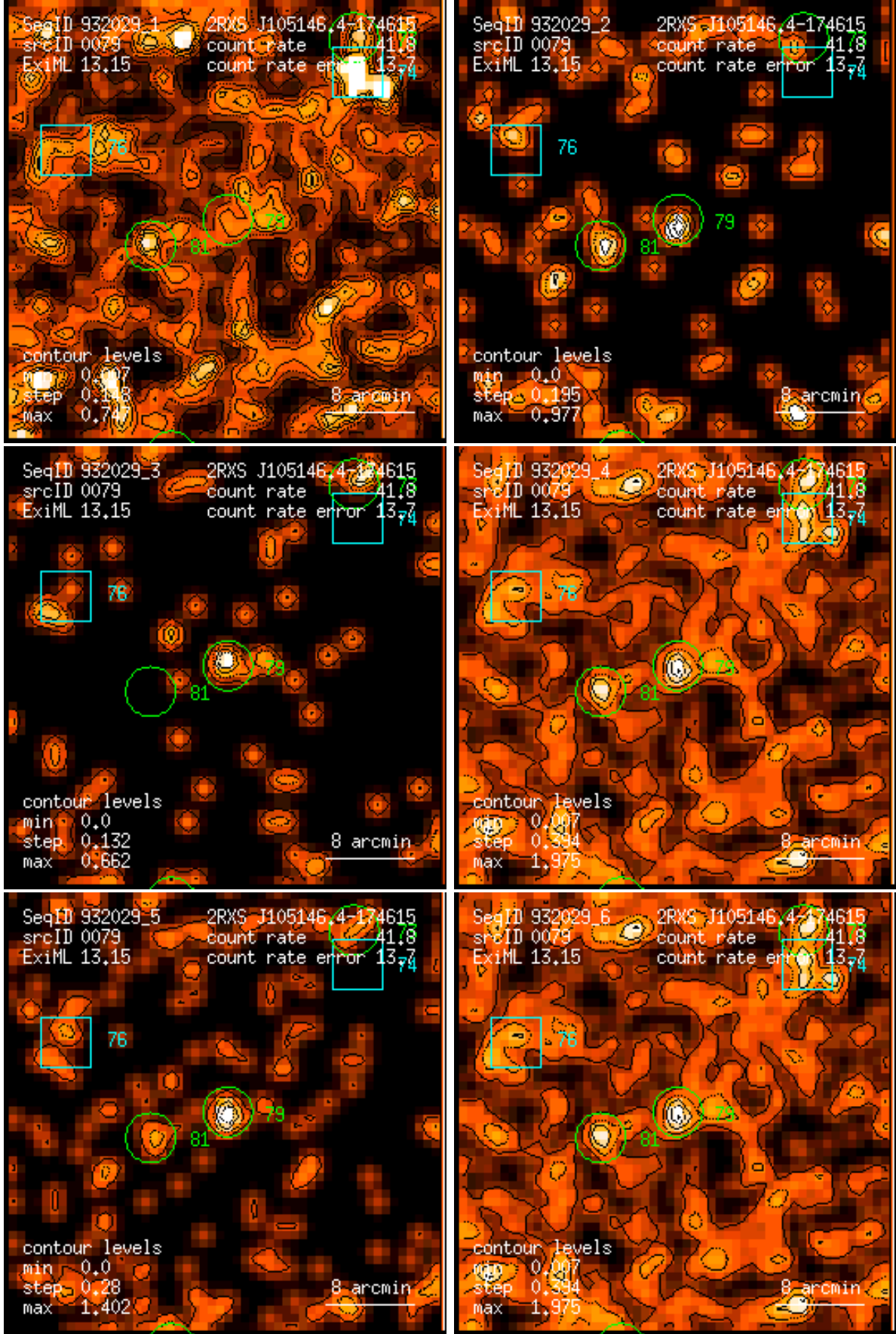
Figure 79: RASS 932029: detection 0079: band rate images, Gaussian filter: (1) PSPC channels 11 – 41, (2) 52 – 90, (3) 91 – 201, (4) 11 – 235, (5) 52 – 201, (6) 11 – 201. Broad band rates in counts/ks. Band rate contour levels in counts/ks/arcmin 2 .
