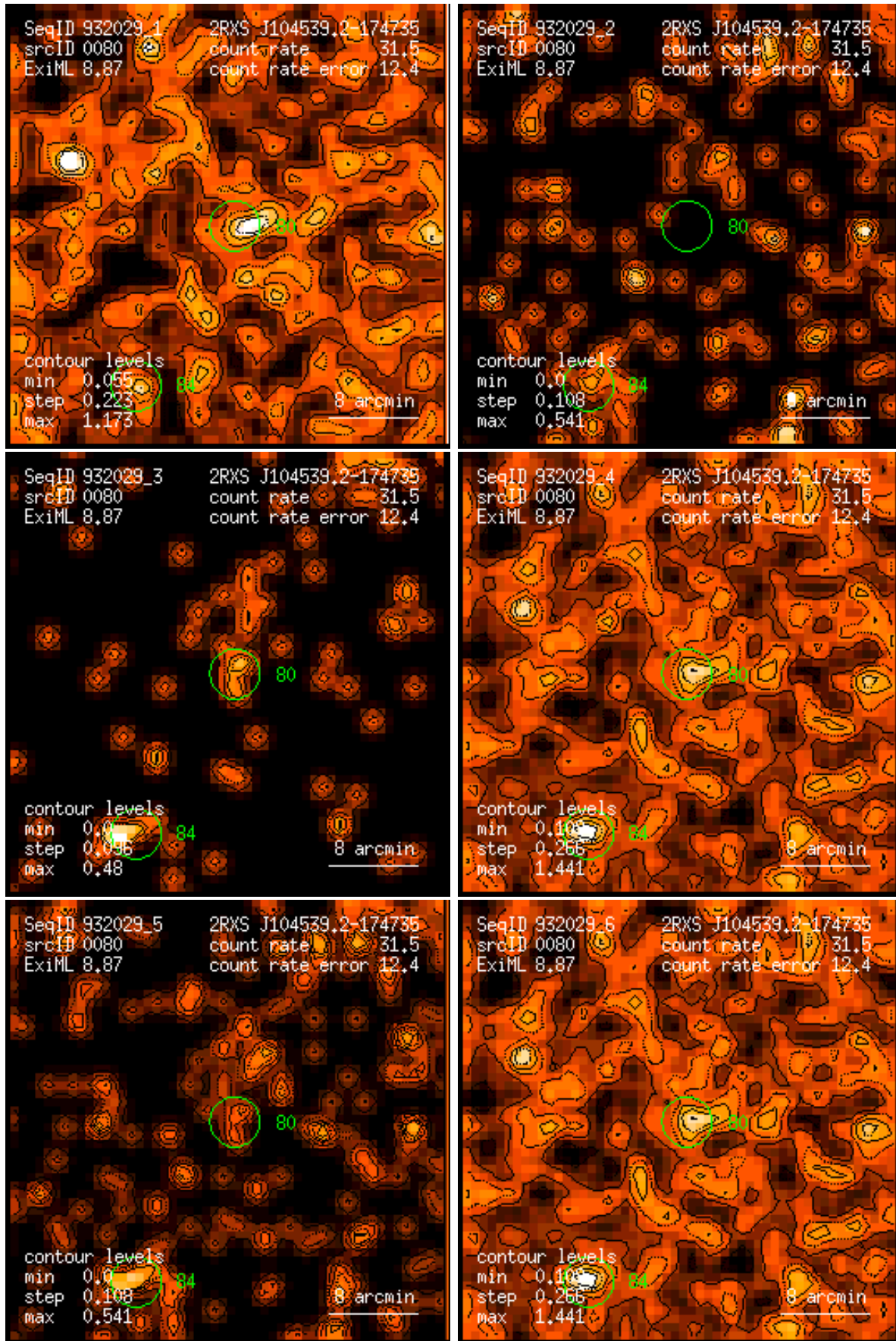
Figure 80: RASS 932029: detection 0080: band rate images, Gaussian filter: (1) PSPC channels 11 – 41, (2) 52 – 90, (3) 91 – 201, (4) 11 – 235, (5) 52 – 201, (6) 11 – 201. Broad band rates in counts/ks. Band rate contour levels in counts/ks/arcmin 2 .
