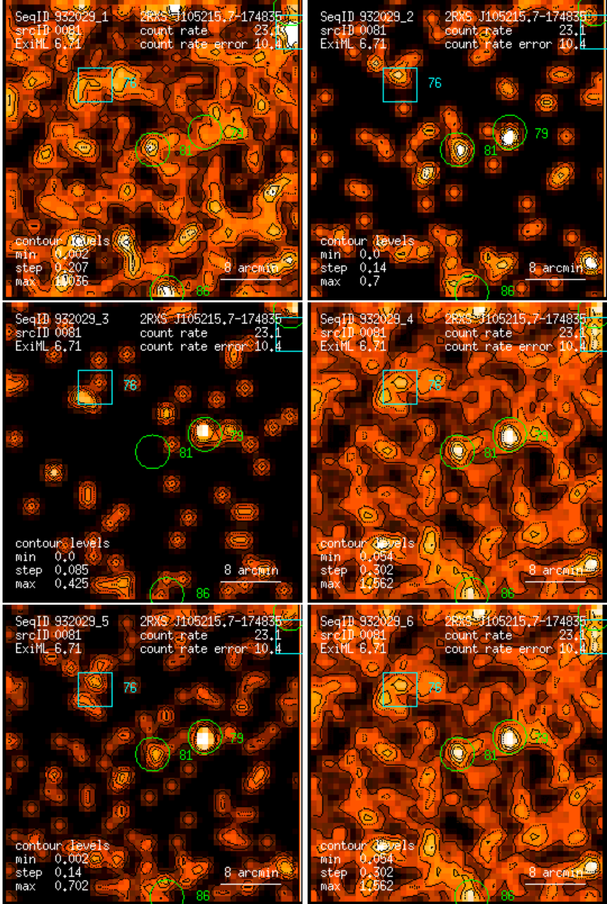
Figure 81: RASS 932029: detection 0081: band rate images, Gaussian filter: (1) PSPC channels 11 – 41, (2) 52 – 90, (3) 91 – 201, (4) 11 – 235, (5) 52 – 201, (6) 11 – 201. Broad band rates in counts/ks. Band rate contour levels in counts/ks/arcmin 2 .
