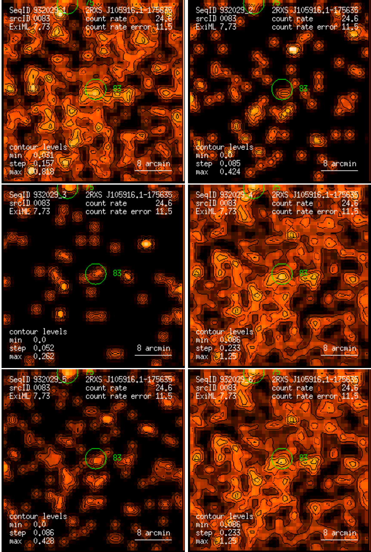
Figure 83: RASS 932029: detection 0083: band rate images, Gaussian filter: (1) PSPC channels 11 – 41, (2) 52 – 90, (3) 91 – 201, (4) 11 – 235, (5) 52 – 201, (6) 11 – 201. Broad band rates in counts/ks. Band rate contour levels in counts/ks/arcmin 2 .
