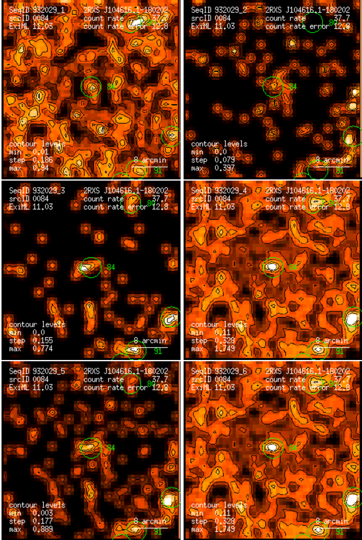
Figure 84: RASS 932029: detection 0084: band rate images, Gaussian filter: (1) PSPC channels 11 – 41, (2) 52 – 90, (3) 91 – 201, (4) 11 – 235, (5) 52 – 201, (6) 11 – 201. Broad band rates in counts/ks. Band rate contour levels in counts/ks/arcmin 2 .
