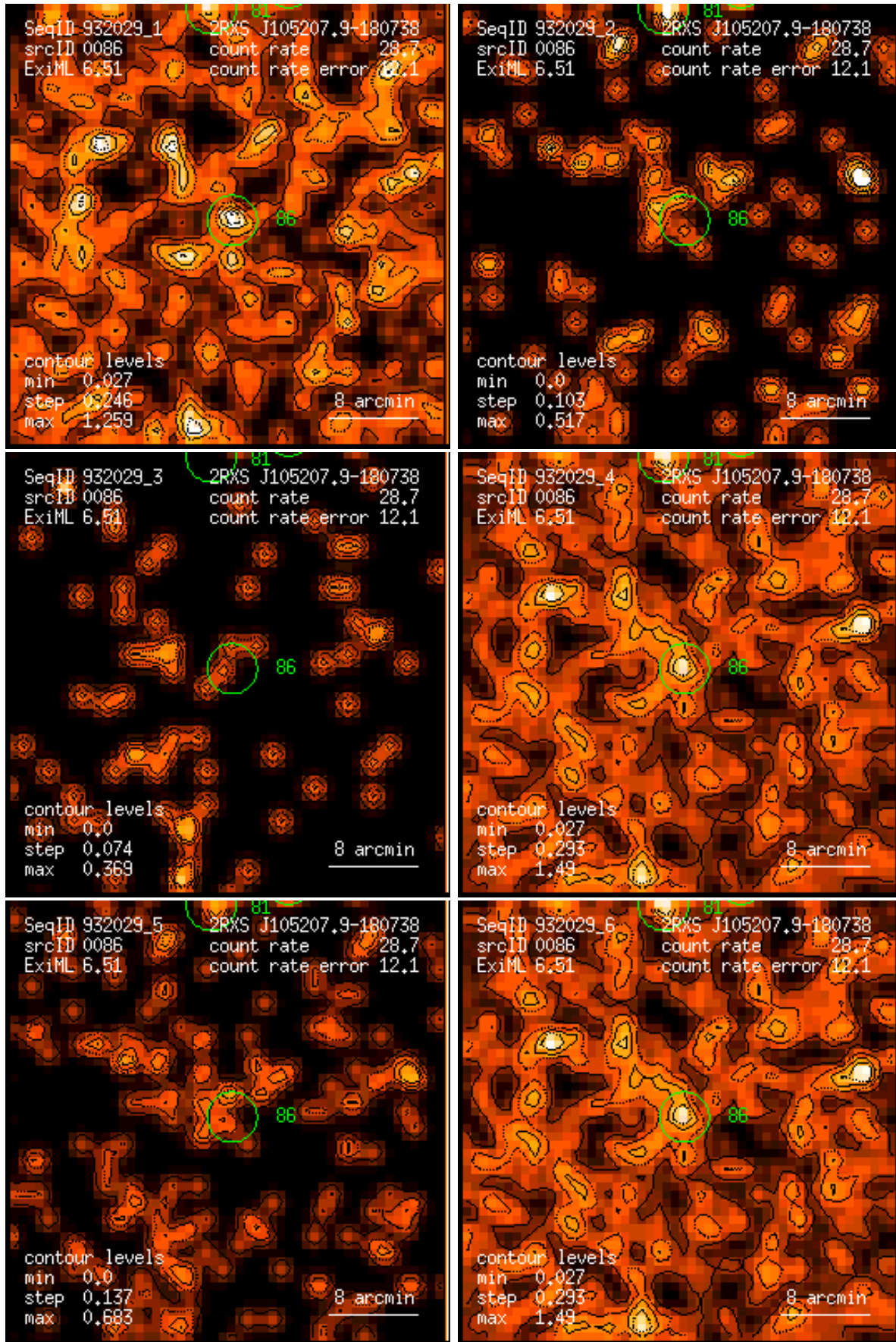
Figure 86: RASS 932029: detection 0086: band rate images, Gaussian filter: (1) PSPC channels 11 – 41, (2) 52 – 90, (3) 91 – 201, (4) 11 – 235, (5) 52 – 201, (6) 11 – 201. Broad band rates in counts/ks. Band rate contour levels in counts/ks/arcmin 2 .
