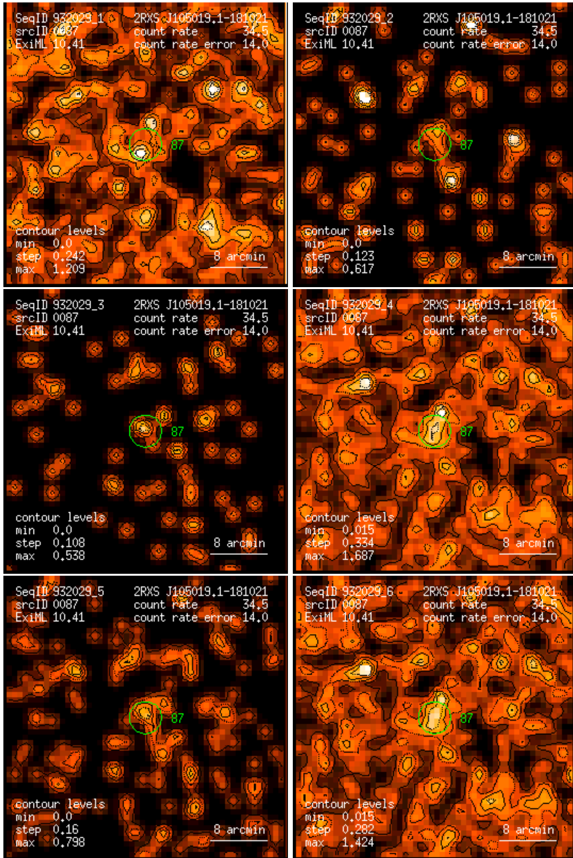
Figure 87: RASS 932029: detection 0087: band rate images, Gaussian filter: (1) PSPC channels 11 – 41, (2) 52 – 90, (3) 91 – 201, (4) 11 – 235, (5) 52 – 201, (6) 11 – 201. Broad band rates in counts/ks. Band rate contour levels in counts/ks/arcmin 2 .
