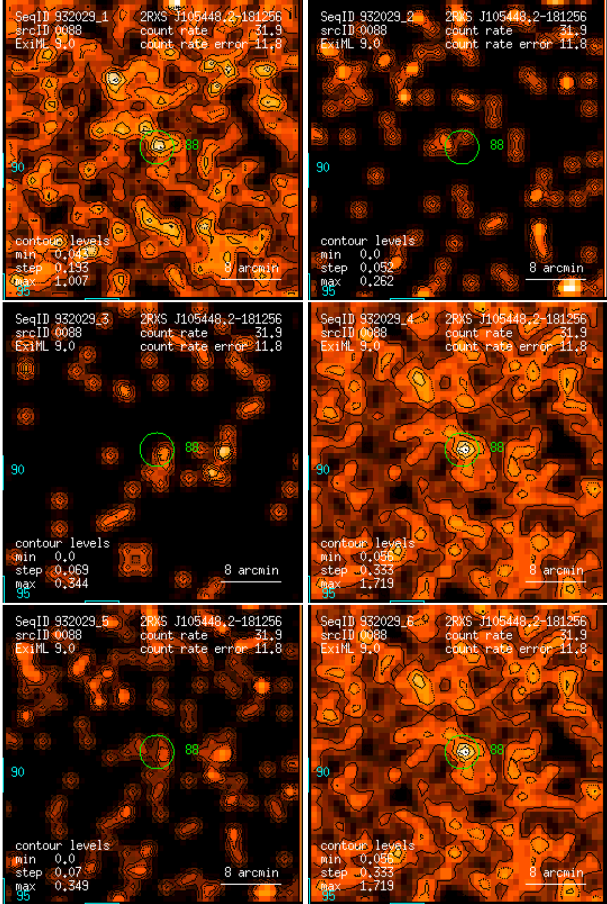
Figure 88: RASS 932029: detection 0088: band rate images, Gaussian filter: (1) PSPC channels 11 – 41, (2) 52 – 90, (3) 91 – 201, (4) 11 – 235, (5) 52 – 201, (6) 11 – 201. Broad band rates in counts/ks. Band rate contour levels in counts/ks/arcmin 2 .
