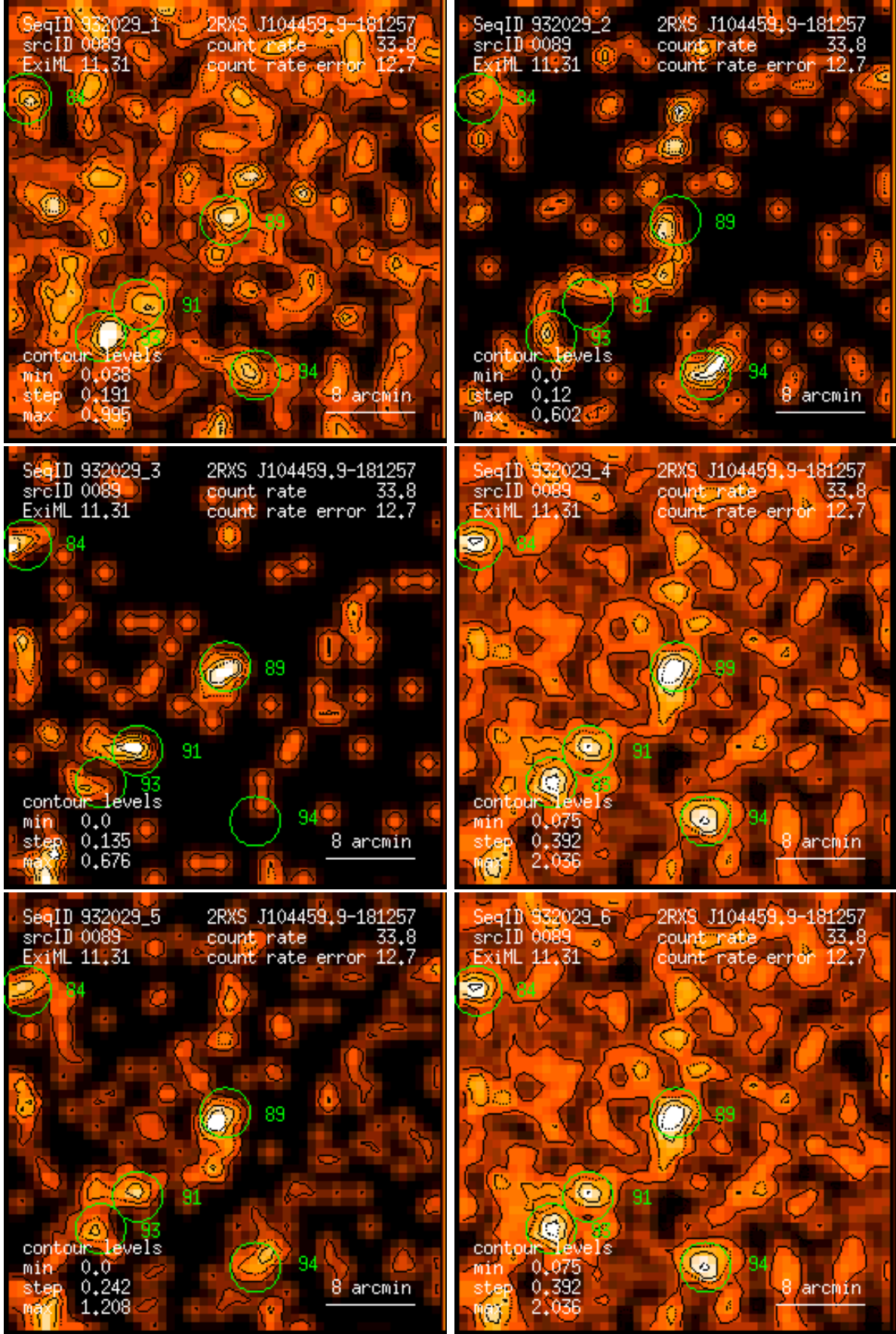
Figure 89: RASS 932029: detection 0089: band rate images, Gaussian filter: (1) PSPC channels 11 – 41, (2) 52 – 90, (3) 91 – 201, (4) 11 – 235, (5) 52 – 201, (6) 11 – 201. Broad band rates in counts/ks. Band rate contour levels in counts/ks/arcmin 2 .
