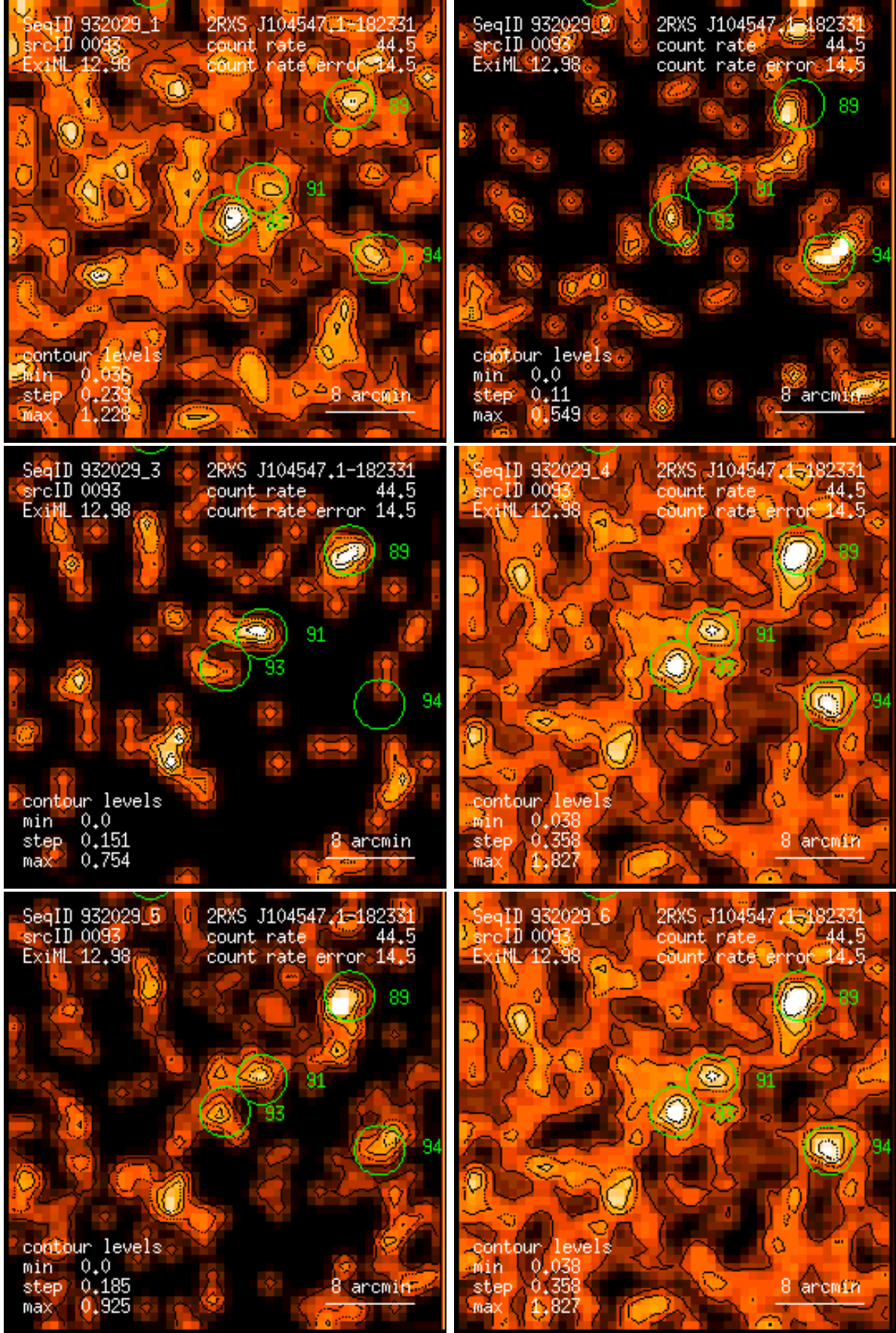
Figure 93: RASS 932029: detection 0093: band rate images, Gaussian filter: (1) PSPC channels 11 – 41, (2) 52 – 90, (3) 91 – 201, (4) 11 – 235, (5) 52 – 201, (6) 11 – 201. Broad band rates in counts/ks. Band rate contour levels in counts/ks/arcmin 2 .
