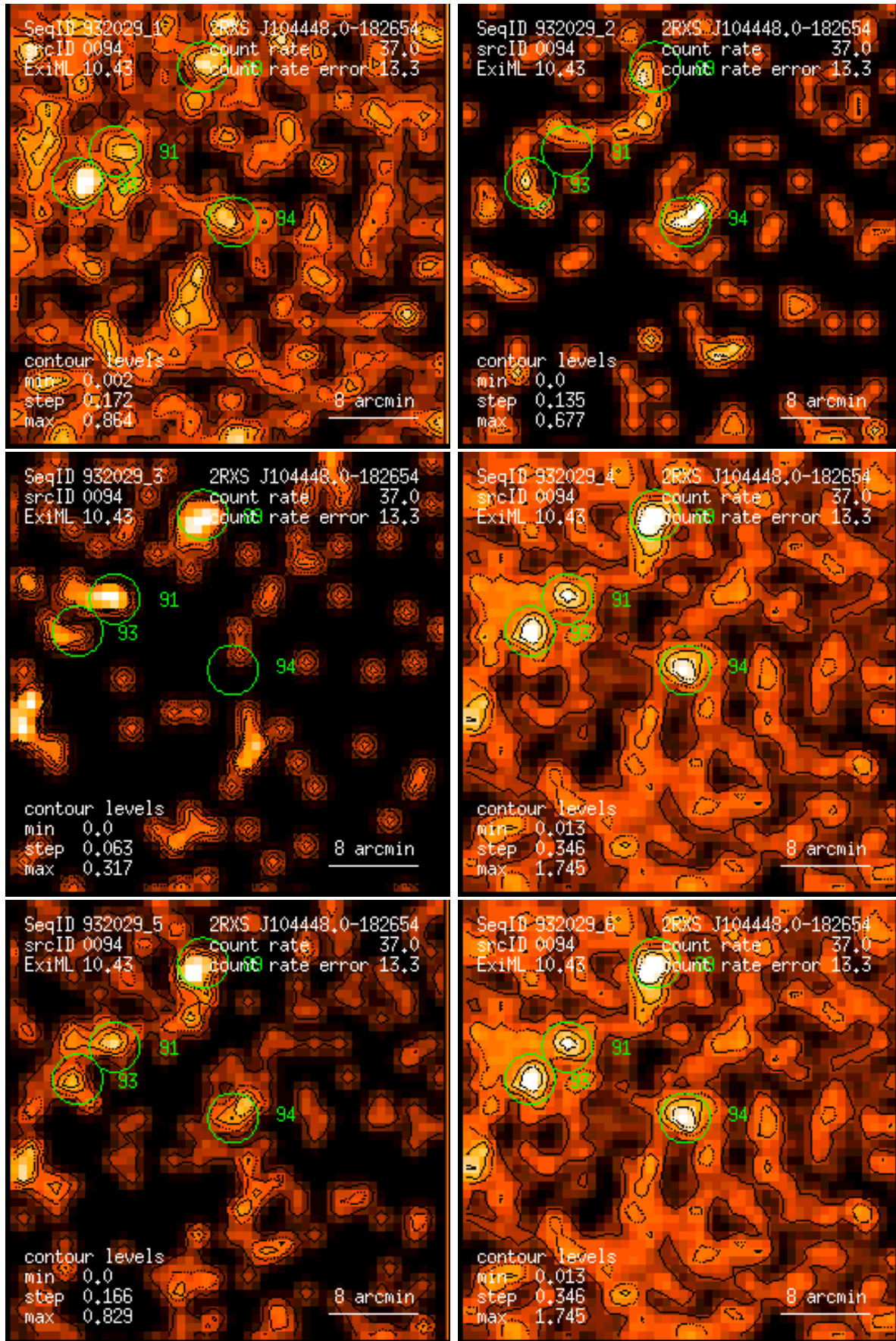
Figure 94: RASS 932029: detection 0094: band rate images, Gaussian filter: (1) PSPC channels 11 – 41, (2) 52 – 90, (3) 91 – 201, (4) 11 – 235, (5) 52 – 201, (6) 11 – 201. Broad band rates in counts/ks. Band rate contour levels in counts/ks/arcmin 2 .
