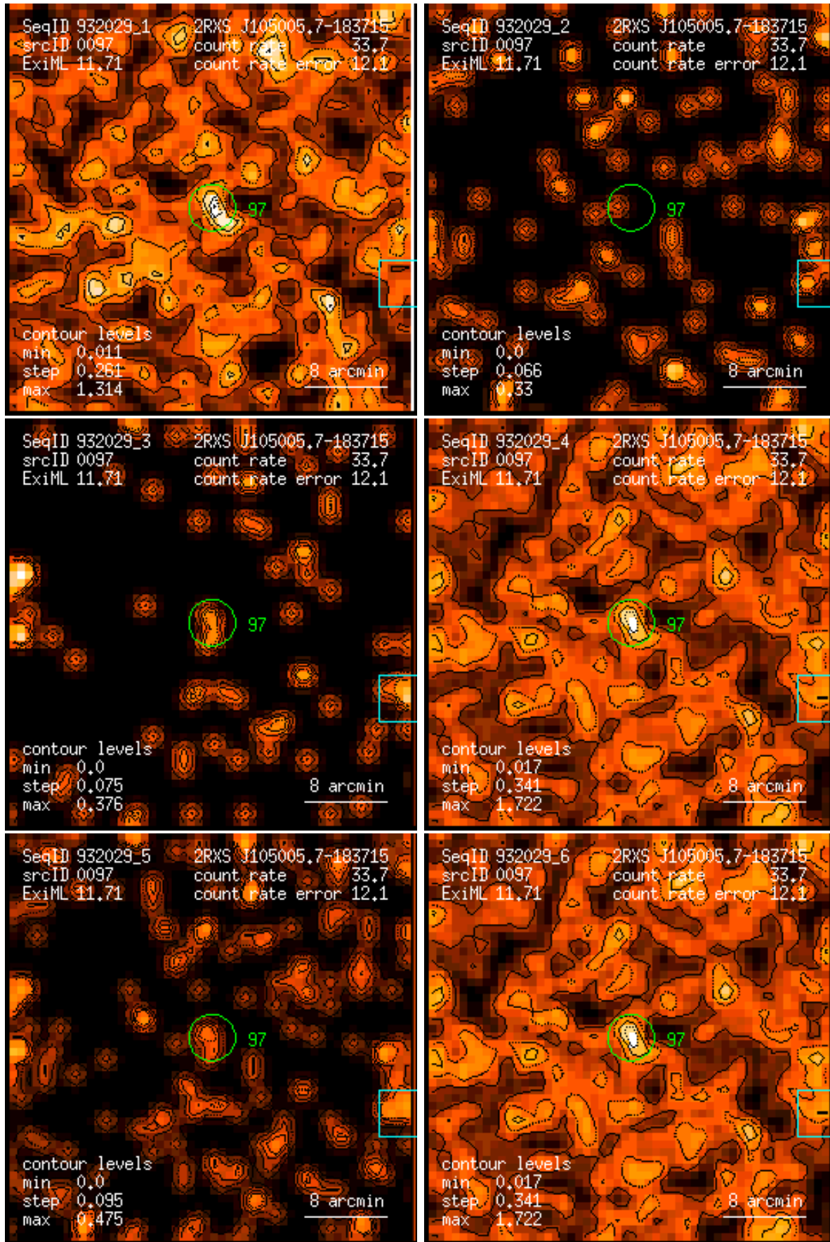
Figure 97: RASS 932029: detection 0097: band rate images, Gaussian filter: (1) PSPC channels 11 – 41, (2) 52 – 90, (3) 91 – 201, (4) 11 – 235, (5) 52 – 201, (6) 11 – 201. Broad band rates in counts/ks. Band rate contour levels in counts/ks/arcmin 2 .
