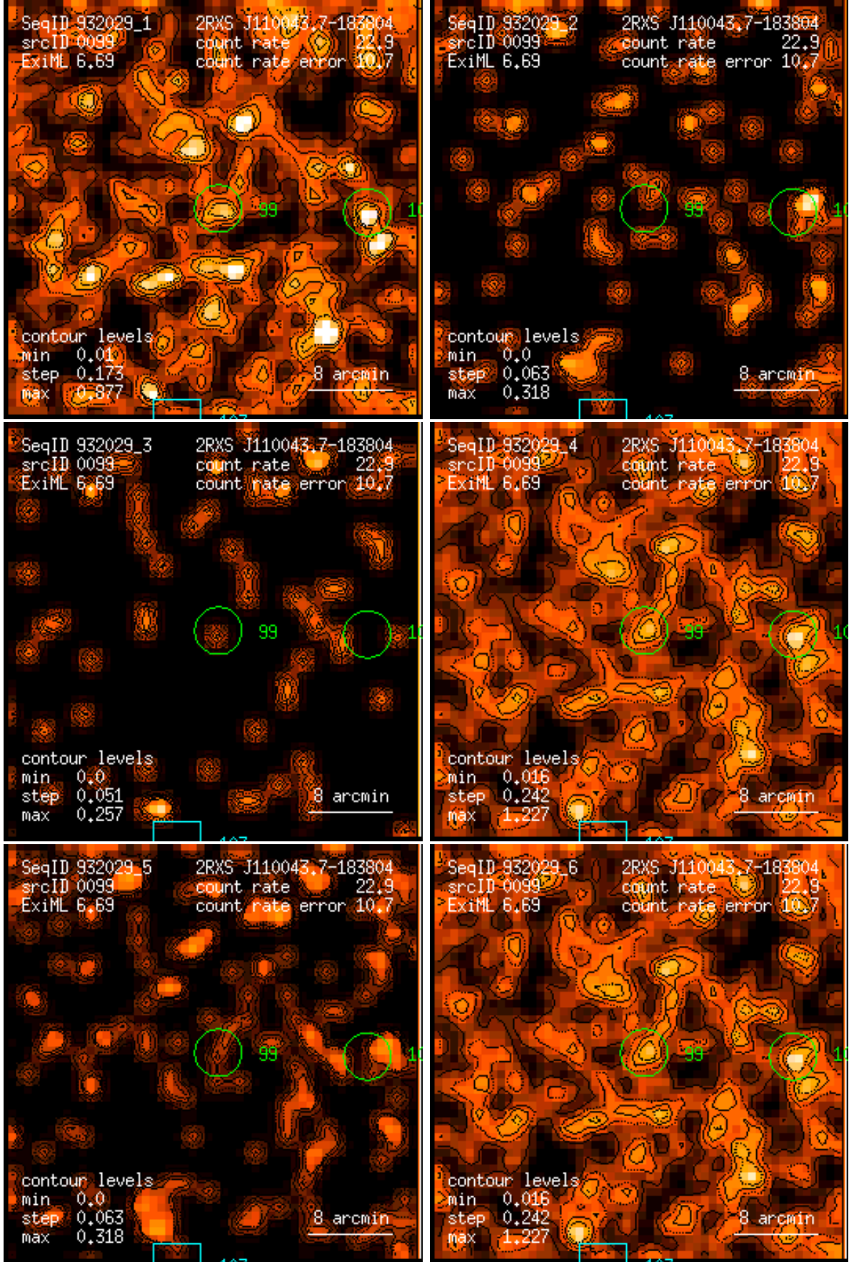
Figure 99: RASS 932029: detection 0099: band rate images, Gaussian filter: (1) PSPC channels 11 – 41, (2) 52 – 90, (3) 91 – 201, (4) 11 – 235, (5) 52 – 201, (6) 11 – 201. Broad band rates in counts/ks. Band rate contour levels in counts/ks/arcmin 2 .
