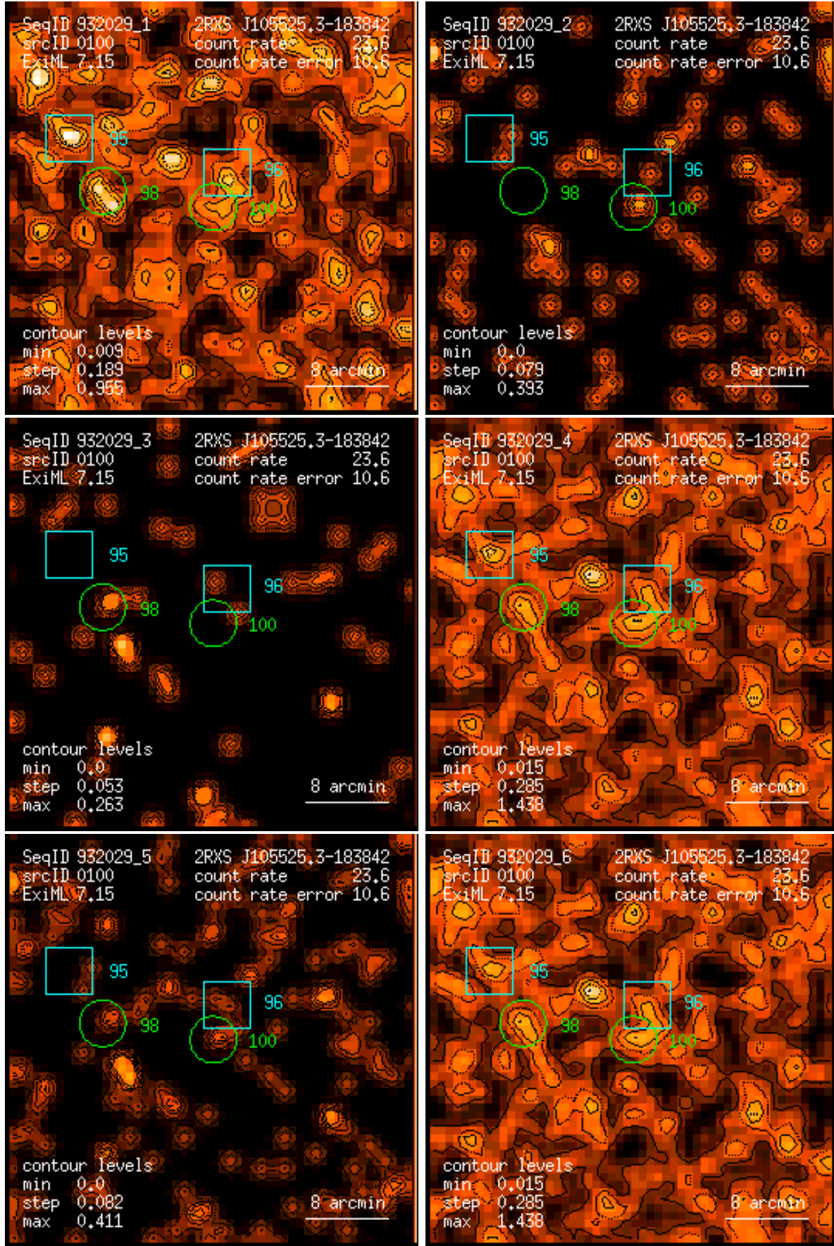
Figure 100: RASS 932029: detection 0100: band rate images, Gaussian filter: (1) PSPC channels 11 – 41, (2) 52 – 90, (3) 91 – 201, (4) 11 – 235, (5) 52 – 201, (6) 11 – 201. Broad band rates in counts/ks. Band rate contour levels in counts/ks/arcmin 2 .
