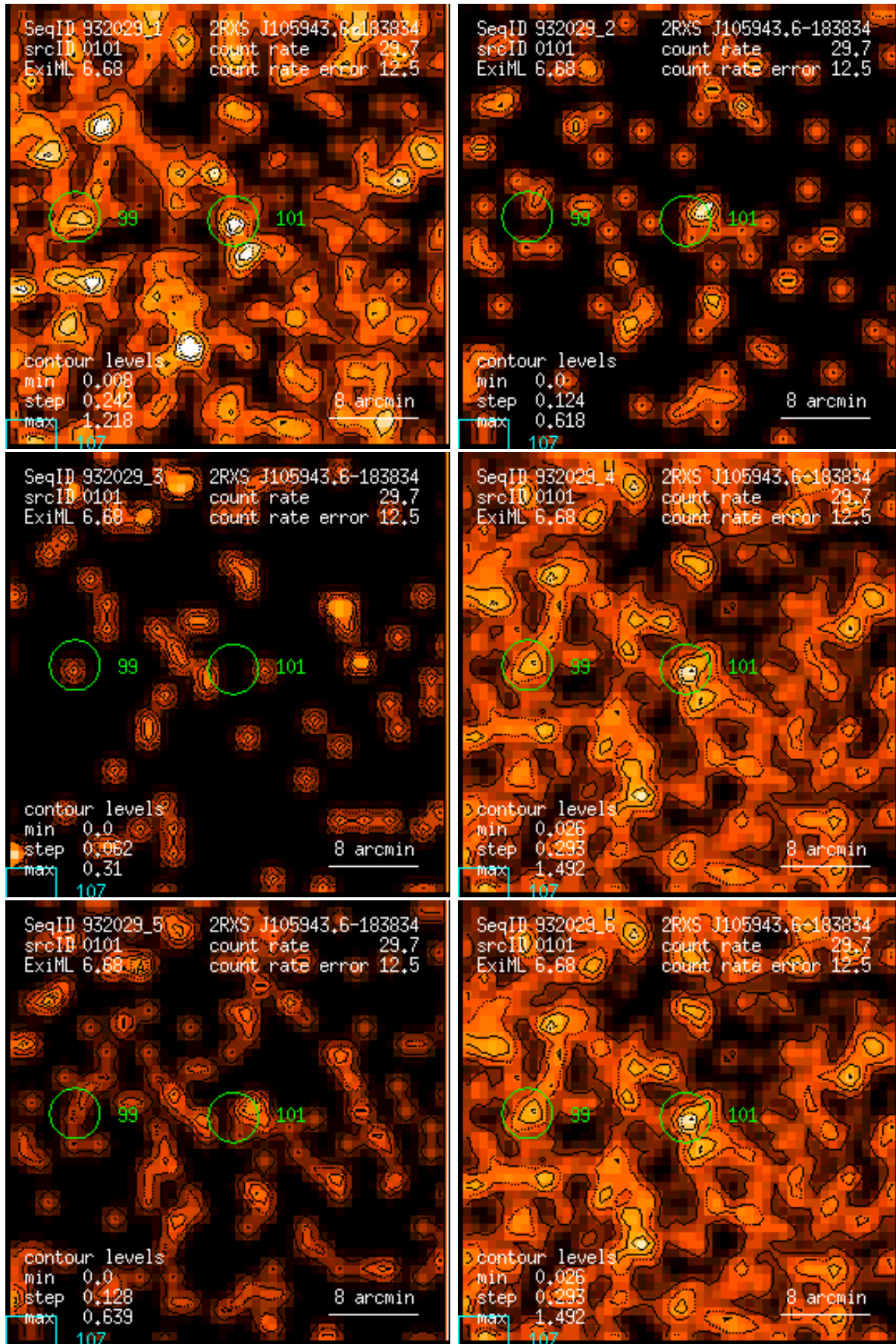
Figure 101: RASS 932029: detection 0101: band rate images, Gaussian filter: (1) PSPC channels 11 – 41, (2) 52 – 90, (3) 91 – 201, (4) 11 – 235, (5) 52 – 201, (6) 11 – 201. Broad band rates in counts/ks. Band rate contour levels in counts/ks/arcmin 2 .
