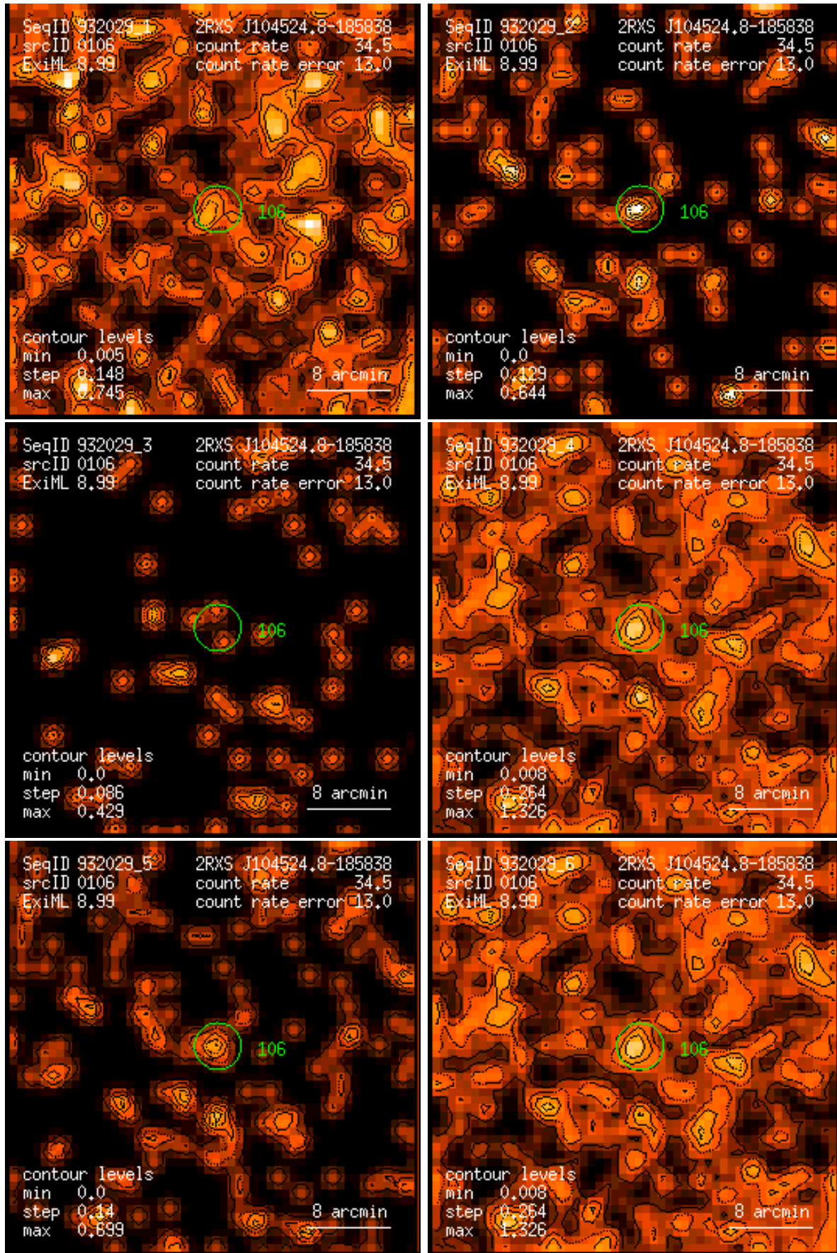
Figure 106: RASS 932029: detection 0106: band rate images, Gaussian filter: (1) PSPC channels 11 – 41, (2) 52 – 90, (3) 91 – 201, (4) 11 – 235, (5) 52 – 201, (6) 11 – 201. Broad band rates in counts/ks. Band rate contour levels in counts/ks/arcmin 2 .
