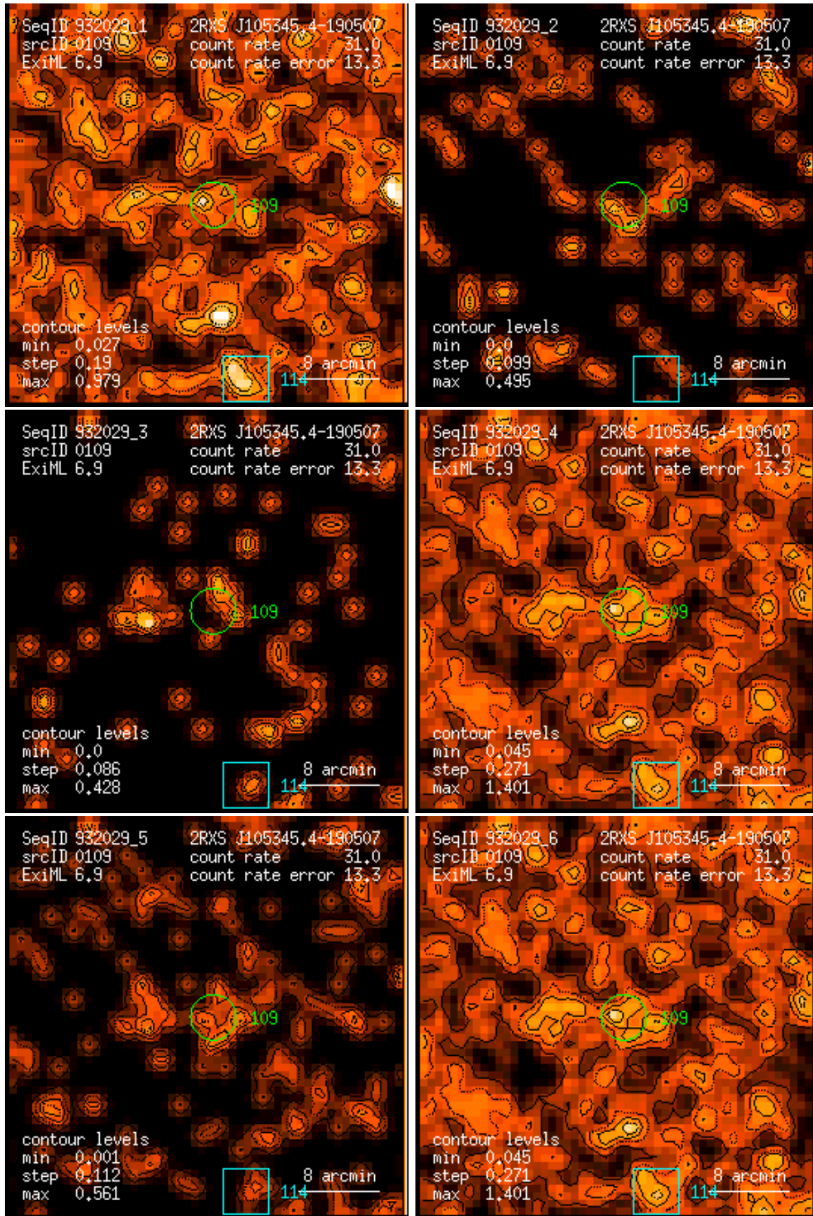
Figure 109: RASS 932029: detection 0109: band rate images, Gaussian filter: (1) PSPC channels 11 – 41, (2) 52 – 90, (3) 91 – 201, (4) 11 – 235, (5) 52 – 201, (6) 11 – 201. Broad band rates in counts/ks. Band rate contour levels in counts/ks/arcmin 2 .
