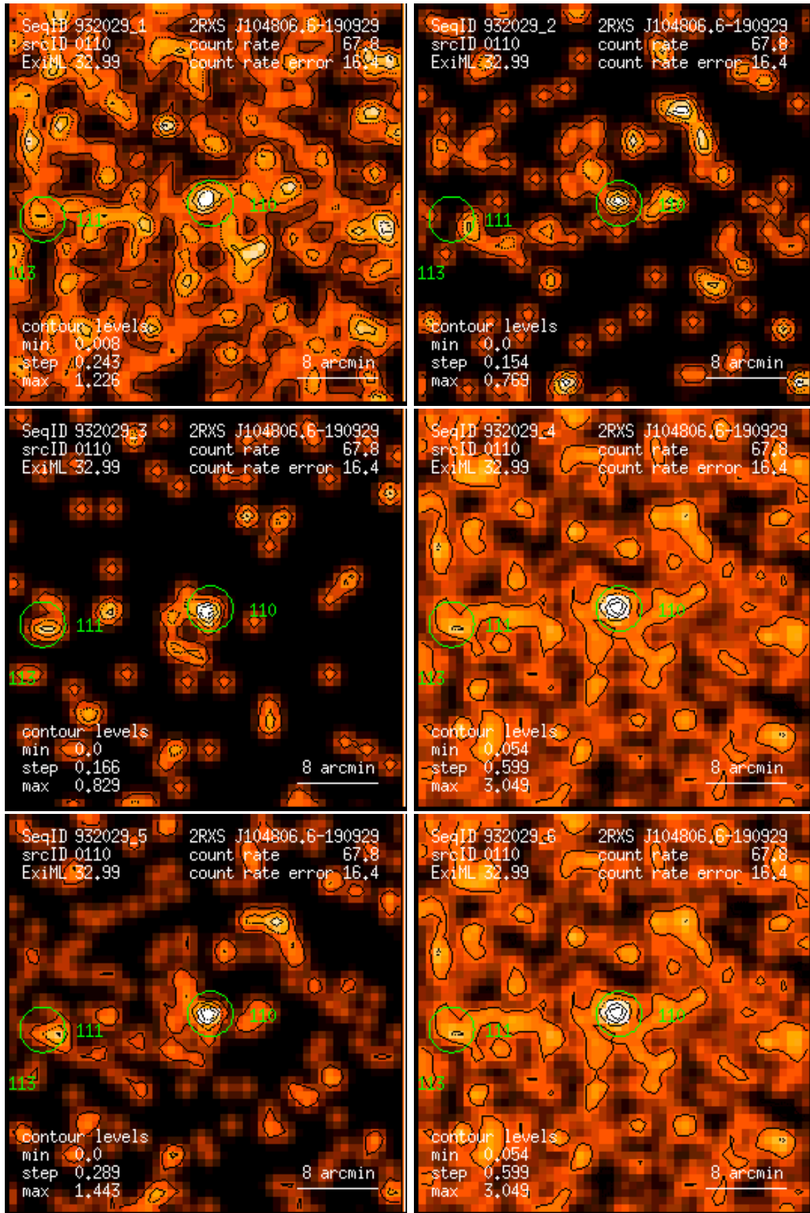
Figure 110: RASS 932029: detection 0110: band rate images, Gaussian filter: (1) PSPC channels 11 – 41, (2) 52 – 90, (3) 91 – 201, (4) 11 – 235, (5) 52 – 201, (6) 11 – 201. Broad band rates in counts/ks. Band rate contour levels in counts/ks/arcmin 2 .
