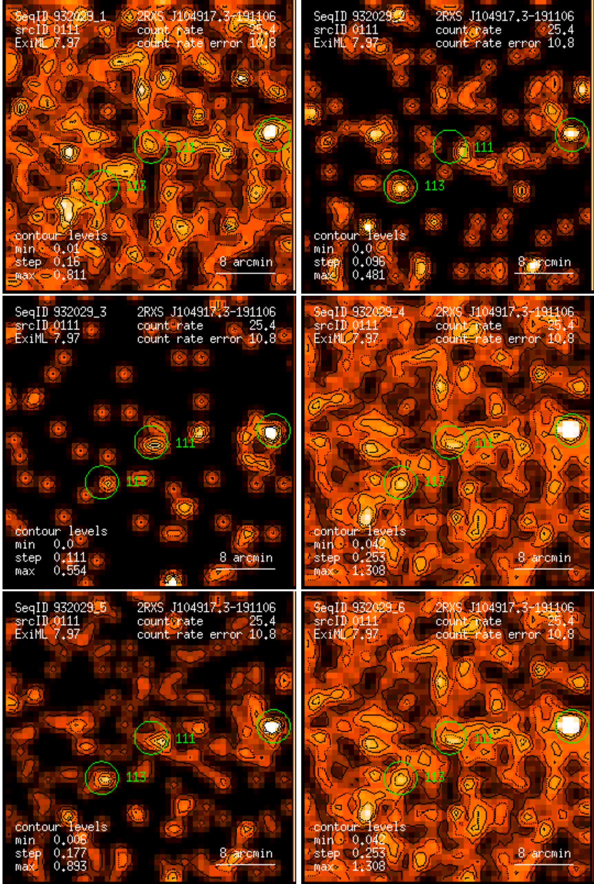
Figure 111: RASS 932029: detection 0111: band rate images, Gaussian filter: (1) PSPC channels 11 – 41, (2) 52 – 90, (3) 91 – 201, (4) 11 – 235, (5) 52 – 201, (6) 11 – 201. Broad band rates in counts/ks. Band rate contour levels in counts/ks/arcmin 2 .
