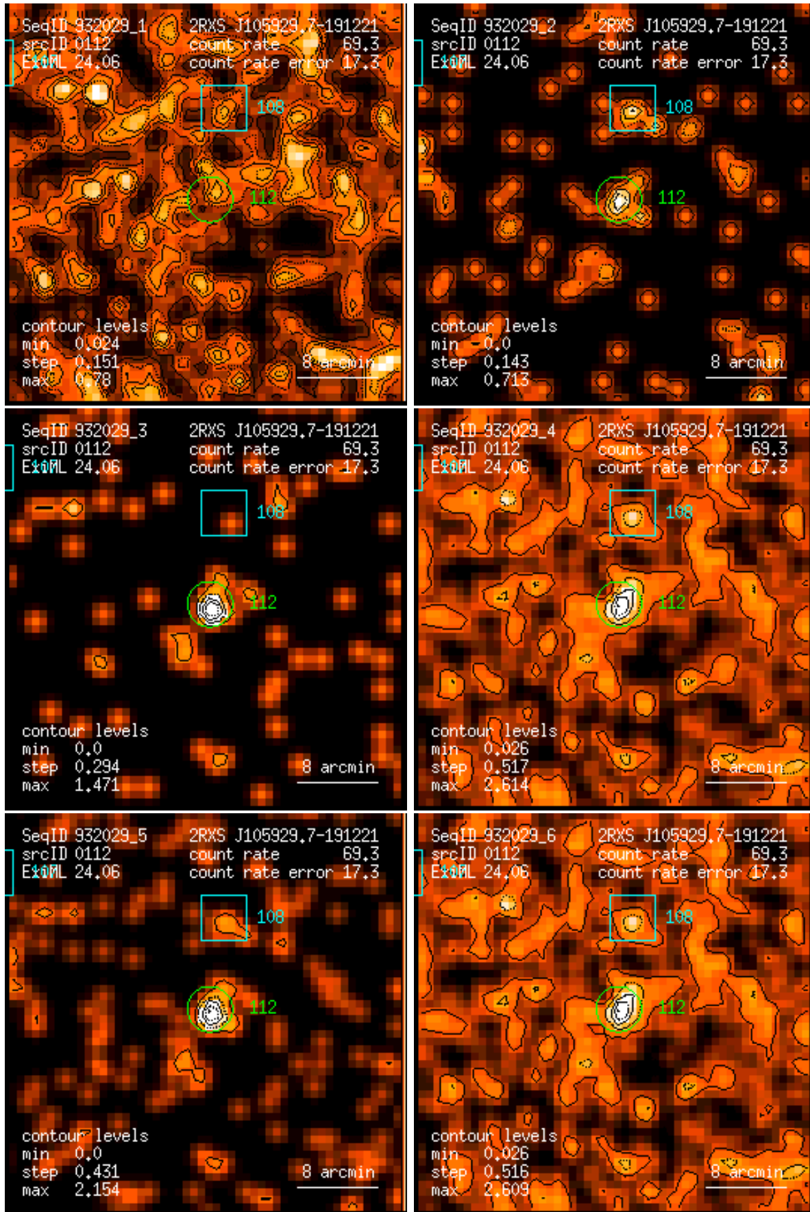
Figure 112: RASS 932029: detection 0112: band rate images, Gaussian filter: (1) PSPC channels 11 – 41, (2) 52 – 90, (3) 91 – 201, (4) 11 – 235, (5) 52 – 201, (6) 11 – 201. Broad band rates in counts/ks. Band rate contour levels in counts/ks/arcmin 2 .
