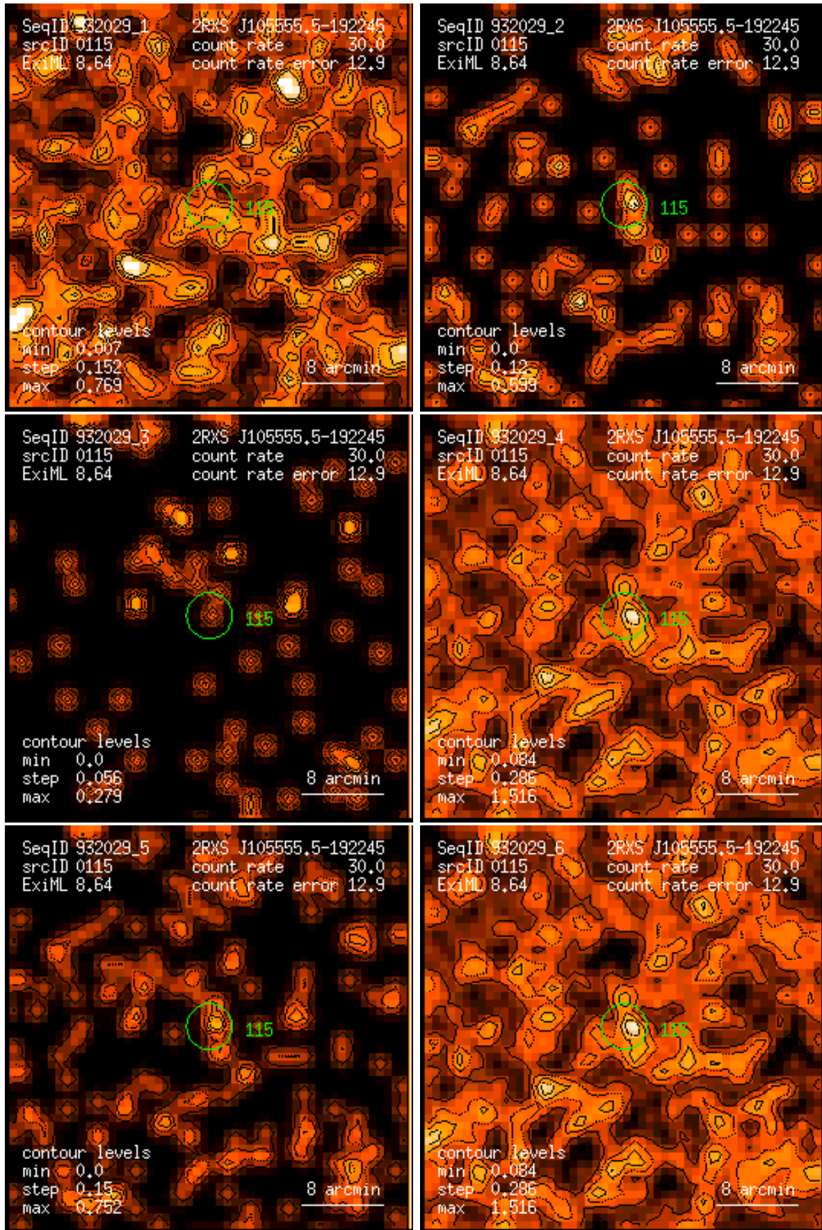
Figure 115: RASS 932029: detection 0115: band rate images, Gaussian filter: (1) PSPC channels 11 – 41, (2) 52 – 90, (3) 91 – 201, (4) 11 – 235, (5) 52 – 201, (6) 11 – 201. Broad band rates in counts/ks. Band rate contour levels in counts/ks/arcmin 2 .
