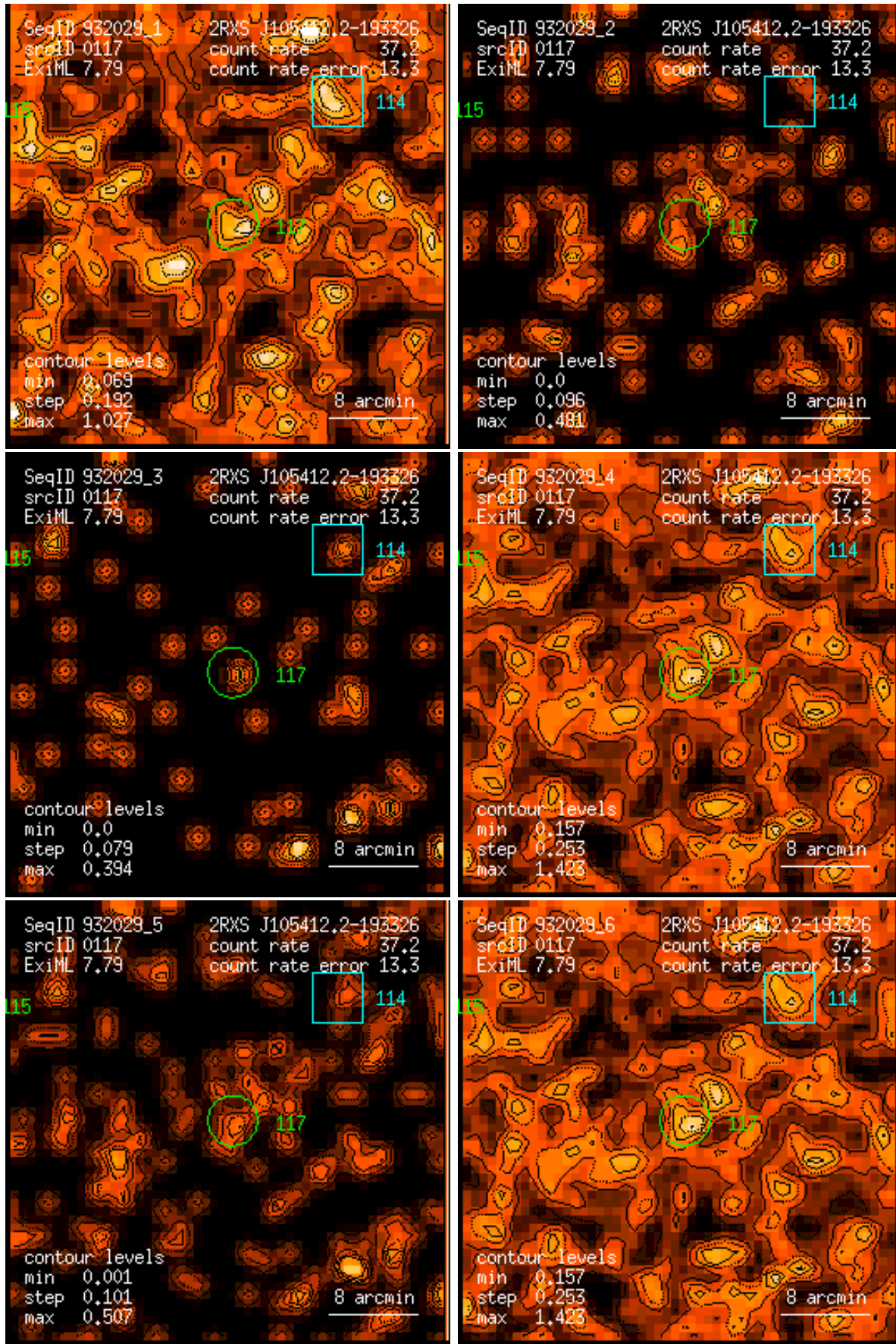
Figure 117: RASS 932029: detection 0117: band rate images, Gaussian filter: (1) PSPC channels 11 – 41, (2) 52 – 90, (3) 91 – 201, (4) 11 – 235, (5) 52 – 201, (6) 11 – 201. Broad band rates in counts/ks. Band rate contour levels in counts/ks/arcmin 2 .
