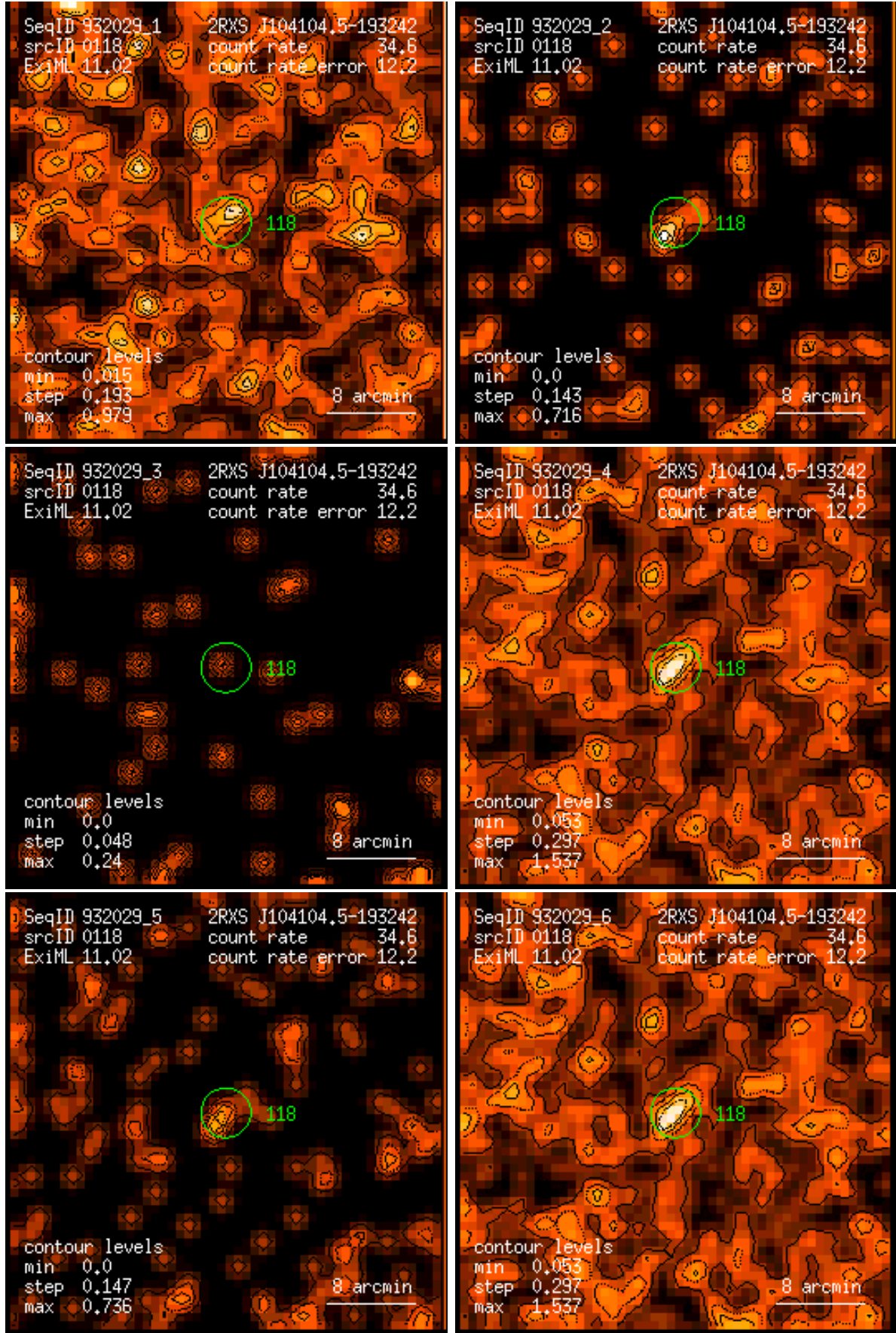
Figure 118: RASS 932029: detection 0118: band rate images, Gaussian filter: (1) PSPC channels 11 – 41, (2) 52 – 90, (3) 91 – 201, (4) 11 – 235, (5) 52 – 201, (6) 11 – 201. Broad band rates in counts/ks. Band rate contour levels in counts/ks/arcmin 2 .
