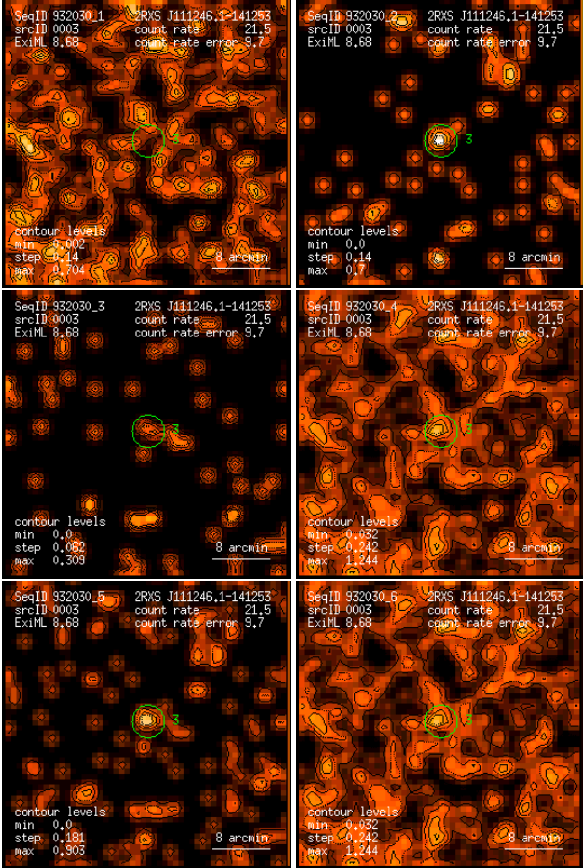
Figure 3: RASS 932030: detection 0003: band rate images, Gaussian filter: (1) PSPC channels 11 – 41, (2) 52 – 90, (3) 91 – 201, (4) 11 – 235, (5) 52 – 201, (6) 11 – 201. Broad band rates in counts/ks. Band rate contour levels in counts/ks/arcmin 2 .
