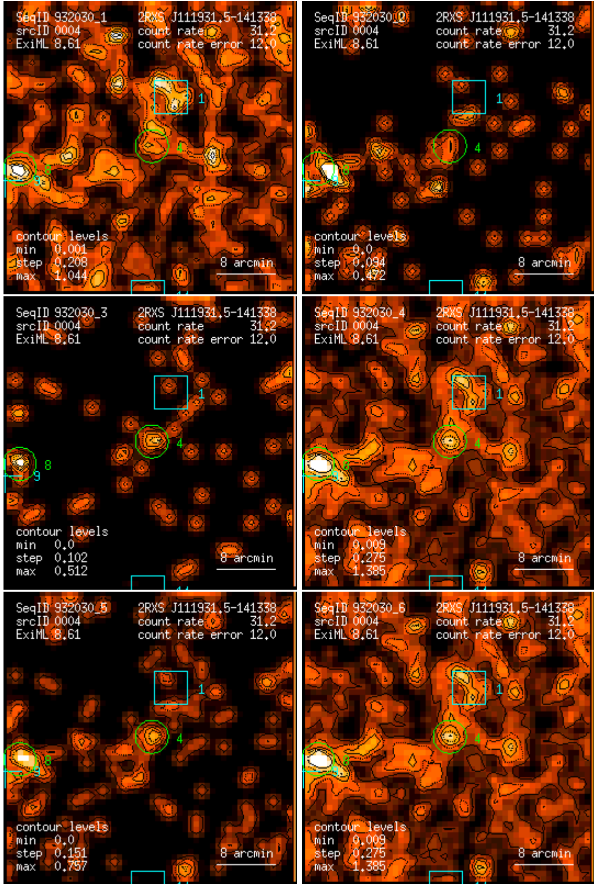
Figure 4: RASS 932030: detection 0004: band rate images, Gaussian filter: (1) PSPC channels 11 – 41, (2) 52 – 90, (3) 91 – 201, (4) 11 – 235, (5) 52 – 201, (6) 11 – 201. Broad band rates in counts/ks. Band rate contour levels in counts/ks/arcmin 2 .
