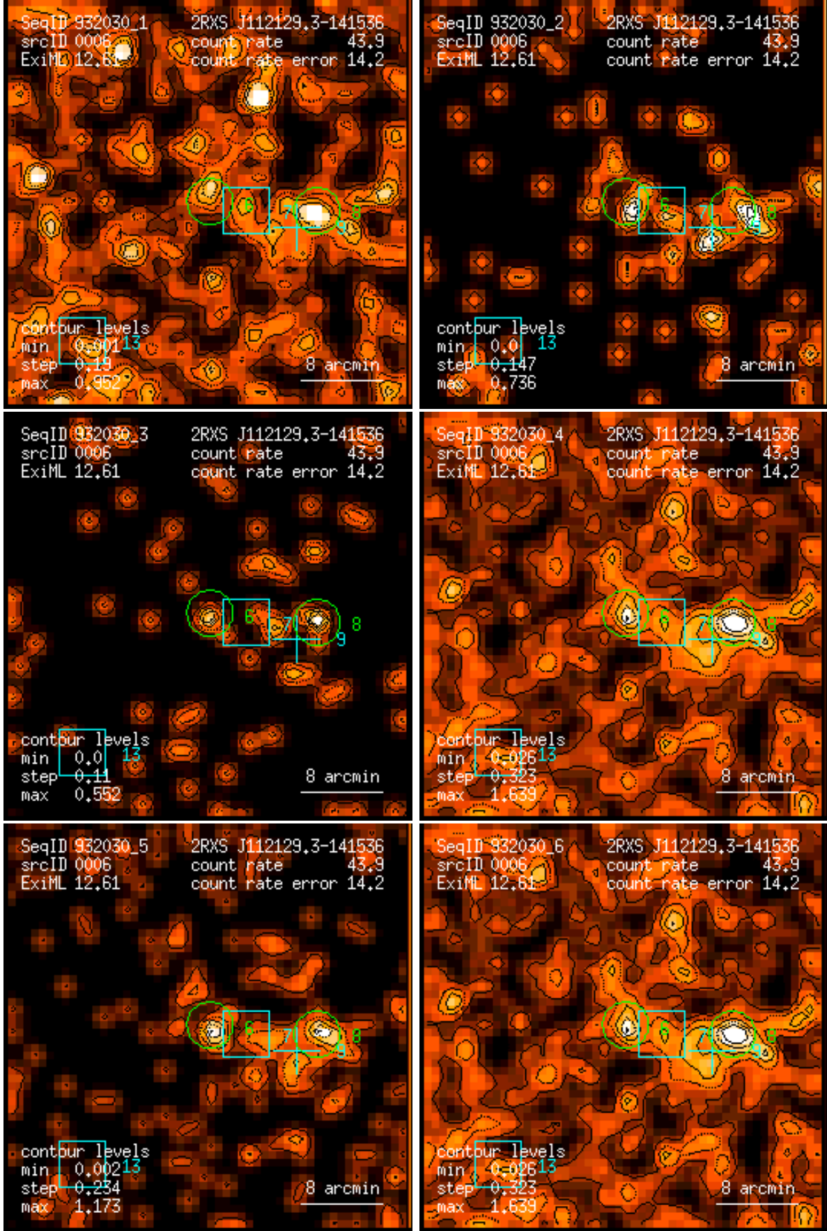
Figure 6: RASS 932030: detection 0006: band rate images, Gaussian filter: (1) PSPC channels 11 – 41, (2) 52 – 90, (3) 91 – 201, (4) 11 – 235, (5) 52 – 201, (6) 11 – 201. Broad band rates in counts/ks. Band rate contour levels in counts/ks/arcmin 2 .
