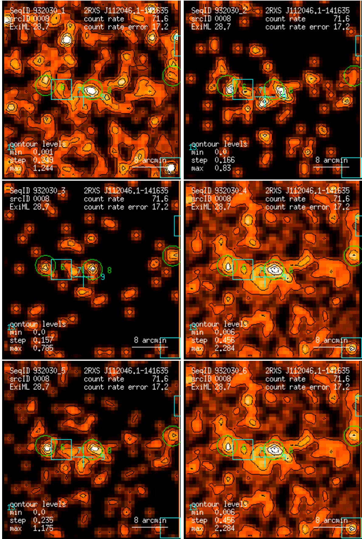
Figure 8: RASS 932030: detection 0008: band rate images, Gaussian filter: (1) PSPC channels 11 – 41, (2) 52 – 90, (3) 91 – 201, (4) 11 – 235, (5) 52 – 201, (6) 11 – 201. Broad band rates in counts/ks. Band rate contour levels in counts/ks/arcmin 2 .
