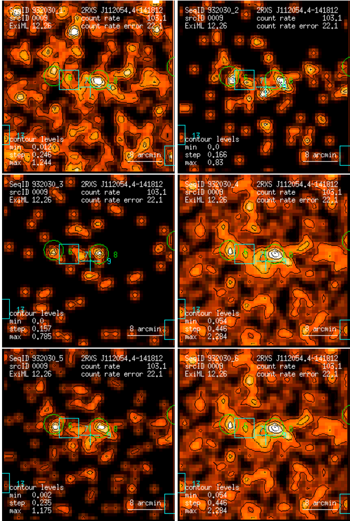
Figure 9: RASS 932030: detection 0009: band rate images, Gaussian filter: (1) PSPC channels 11 – 41, (2) 52 – 90, (3) 91 – 201, (4) 11 – 235, (5) 52 – 201, (6) 11 – 201. Broad band rates in counts/ks. Band rate contour levels in counts/ks/arcmin 2 .
