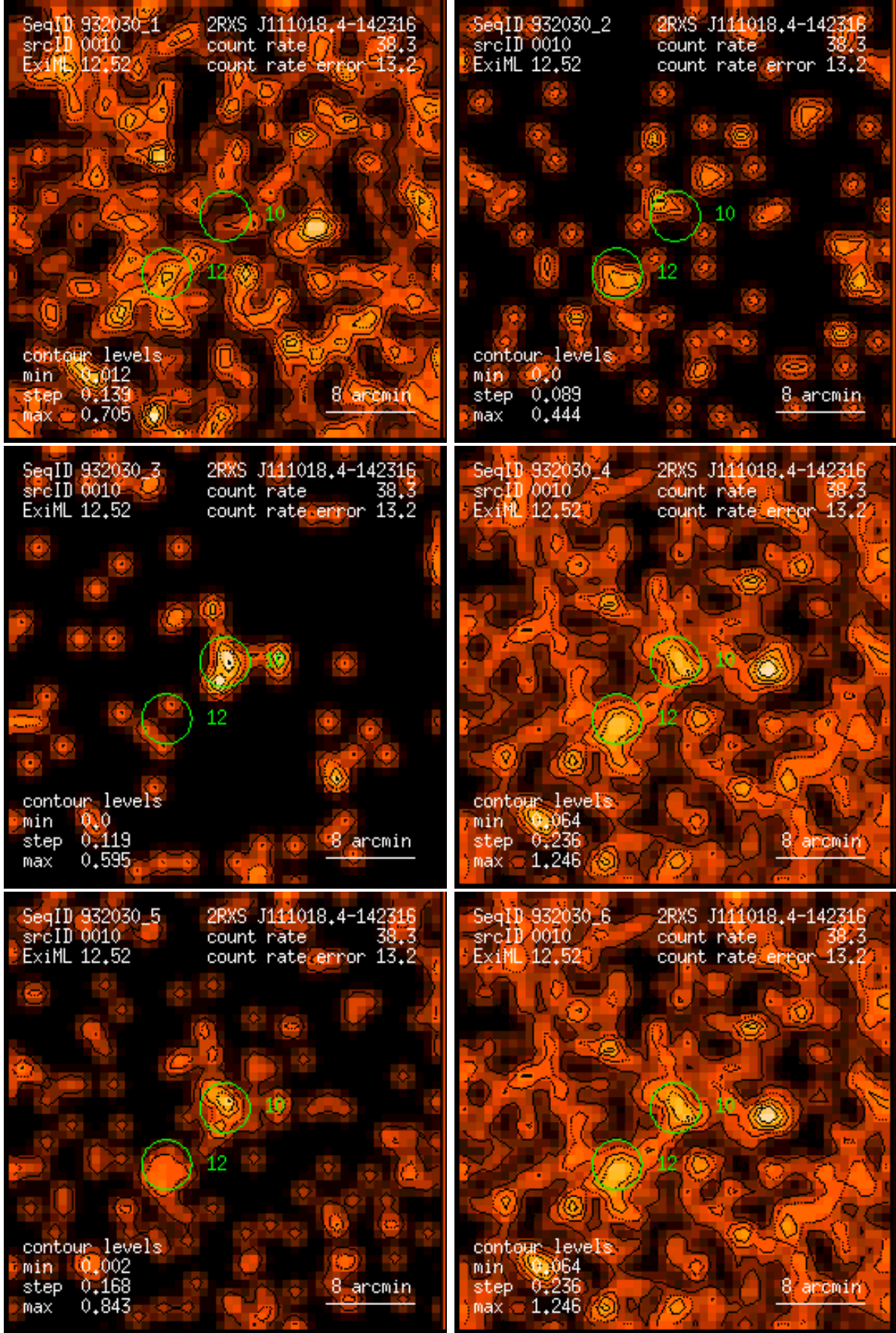
Figure 10: RASS 932030: detection 0010: band rate images, Gaussian filter: (1) PSPC channels 11 – 41, (2) 52 – 90, (3) 91 – 201, (4) 11 – 235, (5) 52 – 201, (6) 11 – 201. Broad band rates in counts/ks. Band rate contour levels in counts/ks/arcmin 2 .
