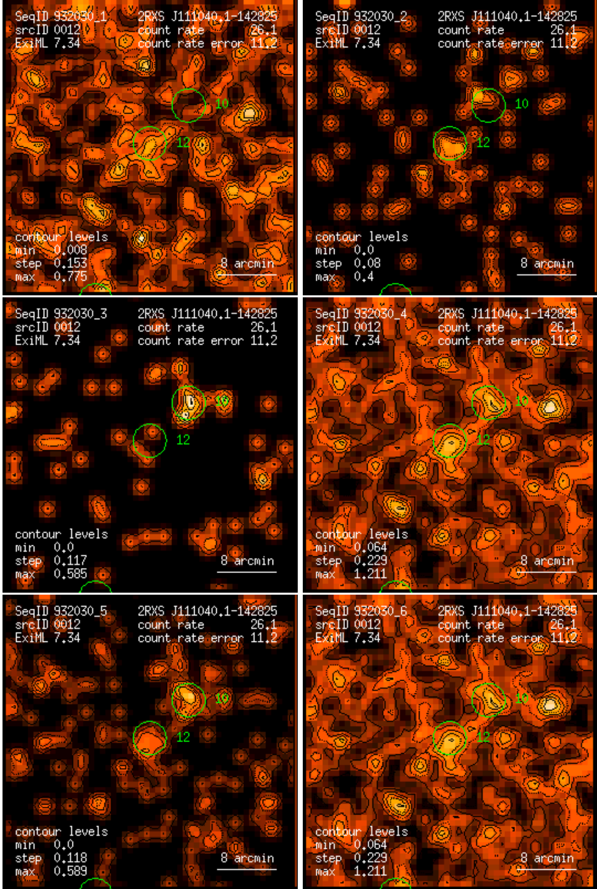
Figure 12: RASS 932030: detection 0012: band rate images, Gaussian filter: (1) PSPC channels 11 – 41, (2) 52 – 90, (3) 91 – 201, (4) 11 – 235, (5) 52 – 201, (6) 11 – 201. Broad band rates in counts/ks. Band rate contour levels in counts/ks/arcmin 2 .
