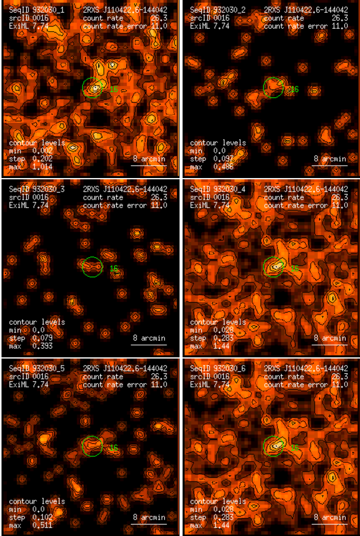
Figure 16: RASS 932030: detection 0016: band rate images, Gaussian filter: (1) PSPC channels 11 – 41, (2) 52 – 90, (3) 91 – 201, (4) 11 – 235, (5) 52 – 201, (6) 11 – 201. Broad band rates in counts/ks. Band rate contour levels in counts/ks/arcmin 2 .
