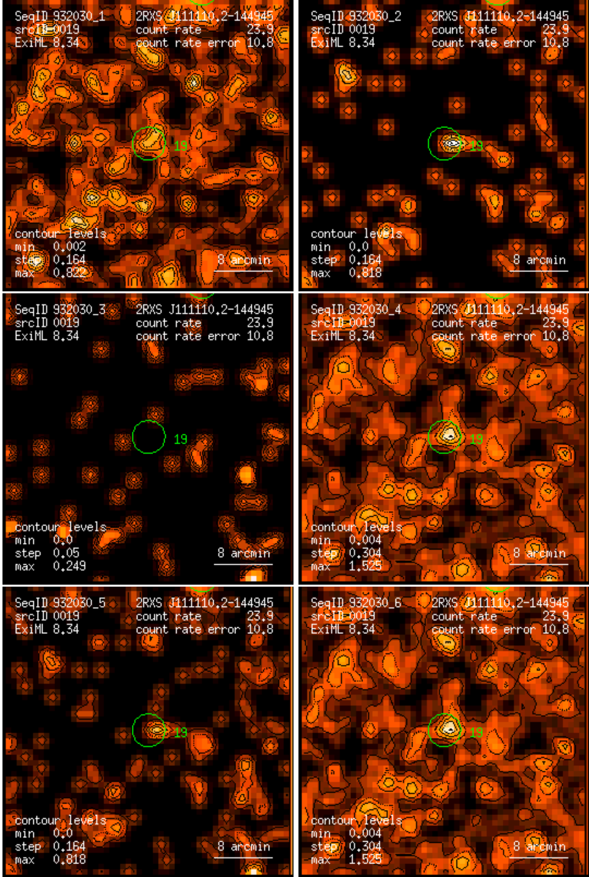
Figure 19: RASS 932030: detection 0019: band rate images, Gaussian filter: (1) PSPC channels 11 – 41, (2) 52 – 90, (3) 91 – 201, (4) 11 – 235, (5) 52 – 201, (6) 11 – 201. Broad band rates in counts/ks. Band rate contour levels in counts/ks/arcmin 2 .
