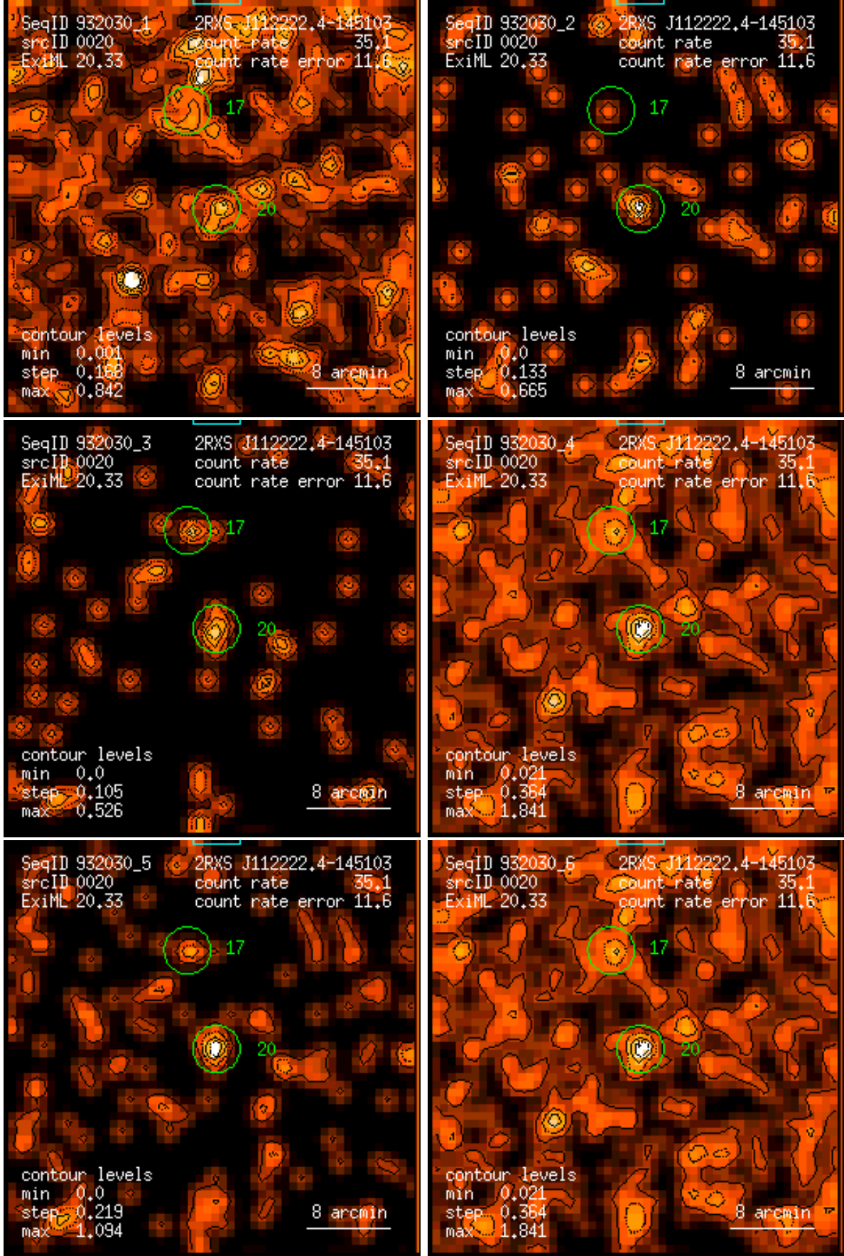
Figure 20: RASS 932030: detection 0020: band rate images, Gaussian filter: (1) PSPC channels 11 – 41, (2) 52 – 90, (3) 91 – 201, (4) 11 – 235, (5) 52 – 201, (6) 11 – 201. Broad band rates in counts/ks. Band rate contour levels in counts/ks/arcmin 2 .
