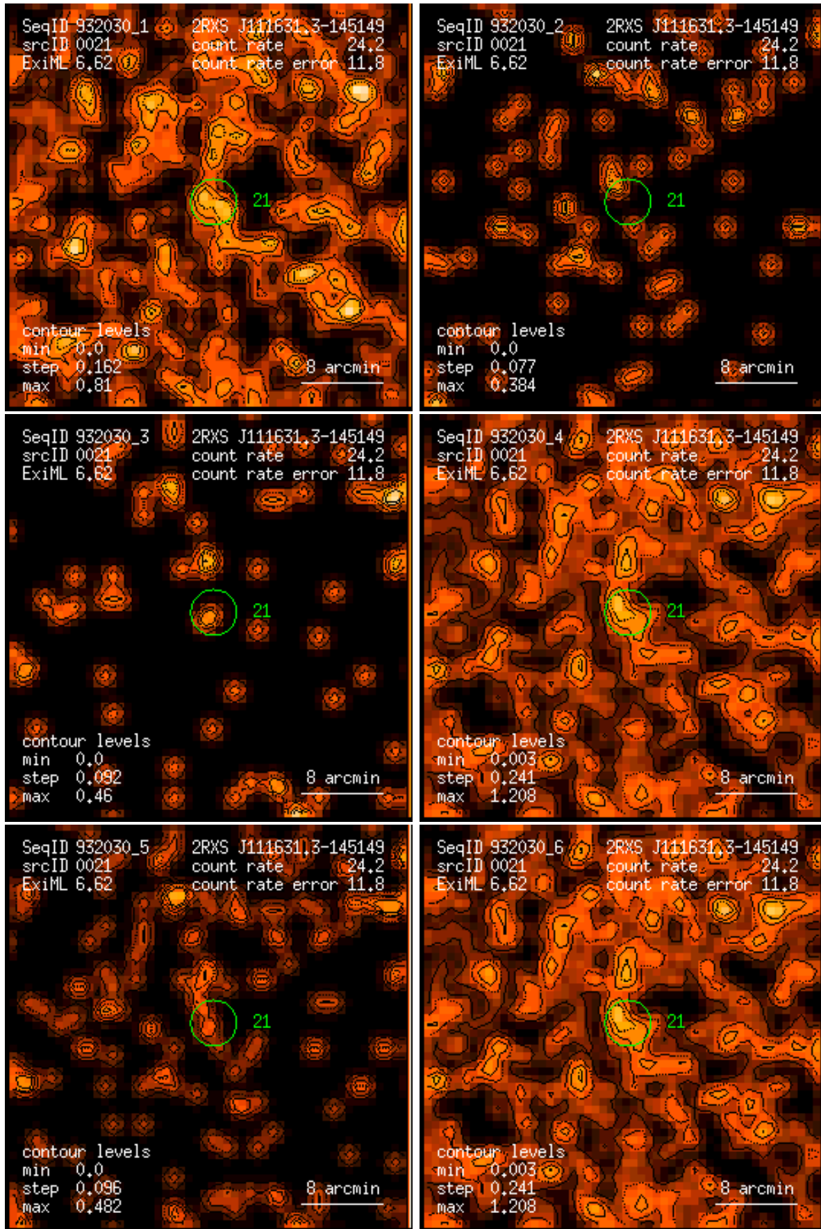
Figure 21: RASS 932030: detection 0021: band rate images, Gaussian filter: (1) PSPC channels 11 – 41, (2) 52 – 90, (3) 91 – 201, (4) 11 – 235, (5) 52 – 201, (6) 11 – 201. Broad band rates in counts/ks. Band rate contour levels in counts/ks/arcmin 2 .
