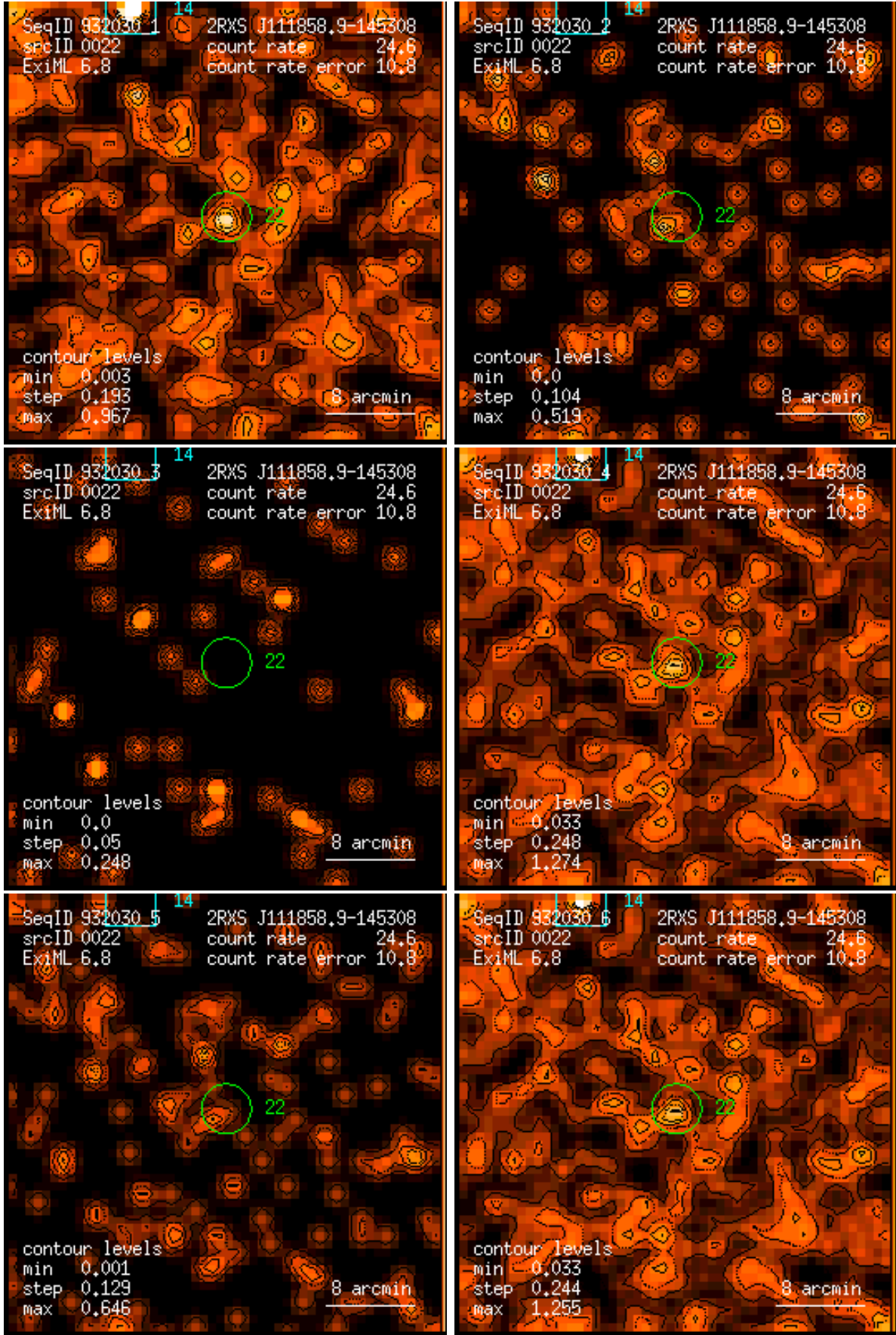
Figure 22: RASS 932030: detection 0022: band rate images, Gaussian filter: (1) PSPC channels 11 – 41, (2) 52 – 90, (3) 91 – 201, (4) 11 – 235, (5) 52 – 201, (6) 11 – 201. Broad band rates in counts/ks. Band rate contour levels in counts/ks/arcmin 2 .
