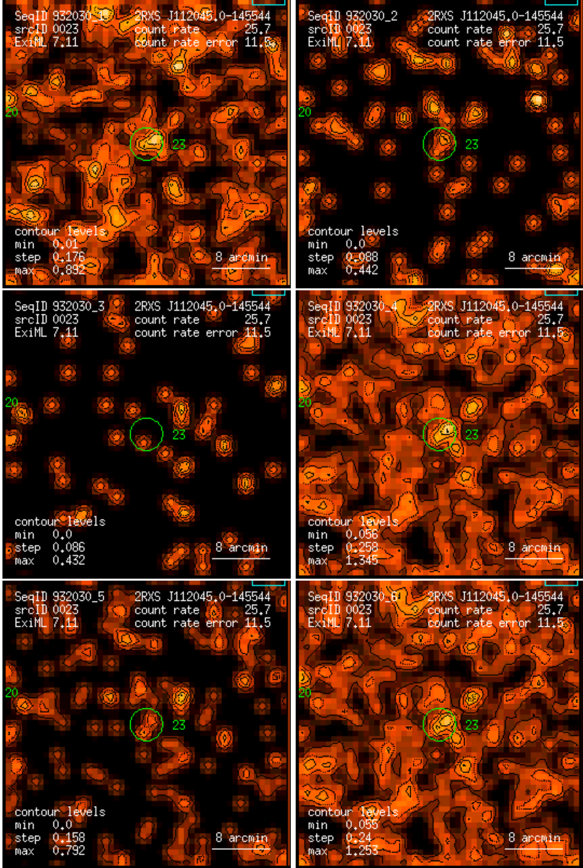
Figure 23: RASS 932030: detection 0023: band rate images, Gaussian filter: (1) PSPC channels 11 – 41, (2) 52 – 90, (3) 91 – 201, (4) 11 – 235, (5) 52 – 201, (6) 11 – 201. Broad band rates in counts/ks. Band rate contour levels in counts/ks/arcmin 2 .
