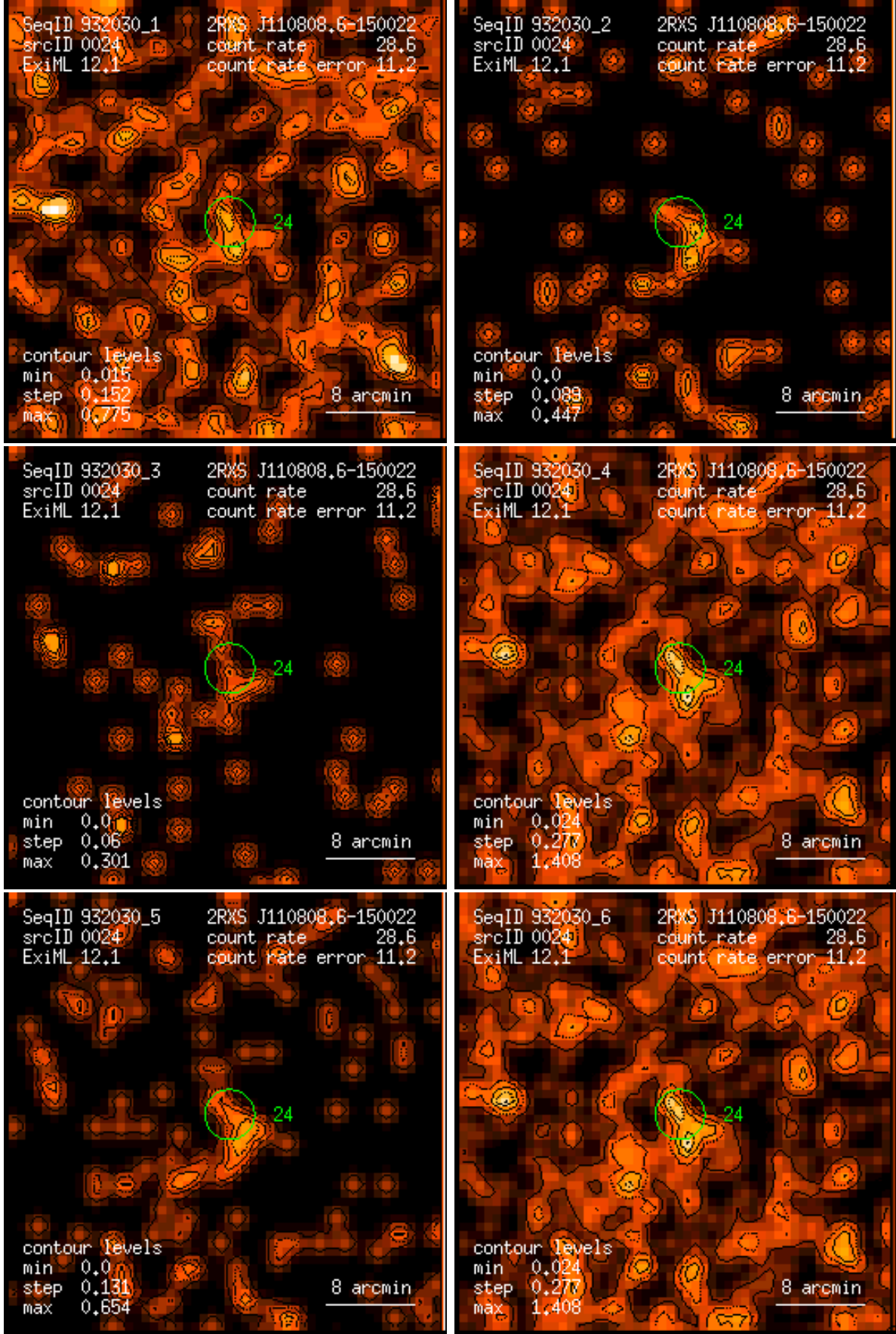
Figure 24: RASS 932030: detection 0024: band rate images, Gaussian filter: (1) PSPC channels 11 – 41, (2) 52 – 90, (3) 91 – 201, (4) 11 – 235, (5) 52 – 201, (6) 11 – 201. Broad band rates in counts/ks. Band rate contour levels in counts/ks/arcmin 2 .
