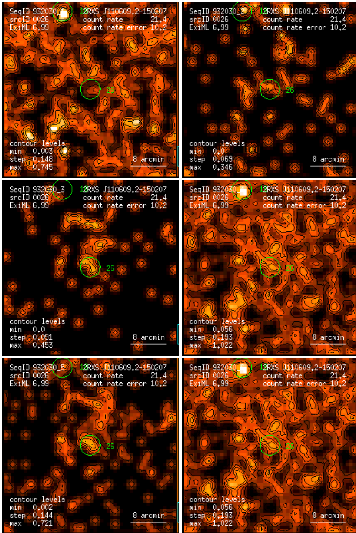
Figure 26: RASS 932030: detection 0026: band rate images, Gaussian filter: (1) PSPC channels 11 – 41, (2) 52 – 90, (3) 91 – 201, (4) 11 – 235, (5) 52 – 201, (6) 11 – 201. Broad band rates in counts/ks. Band rate contour levels in counts/ks/arcmin 2 .
