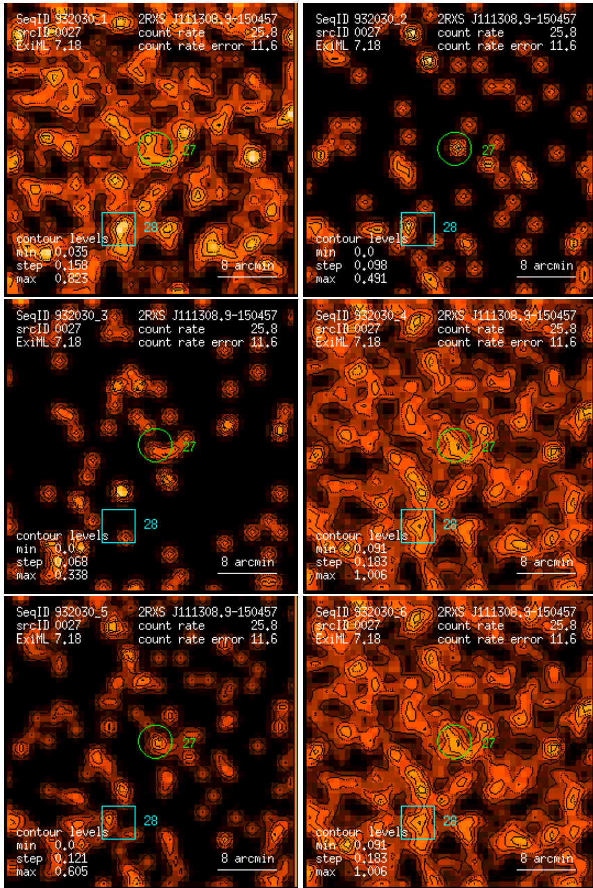
Figure 27: RASS 932030: detection 0027: band rate images, Gaussian filter: (1) PSPC channels 11 – 41, (2) 52 – 90, (3) 91 – 201, (4) 11 – 235, (5) 52 – 201, (6) 11 – 201. Broad band rates in counts/ks. Band rate contour levels in counts/ks/arcmin 2 .
