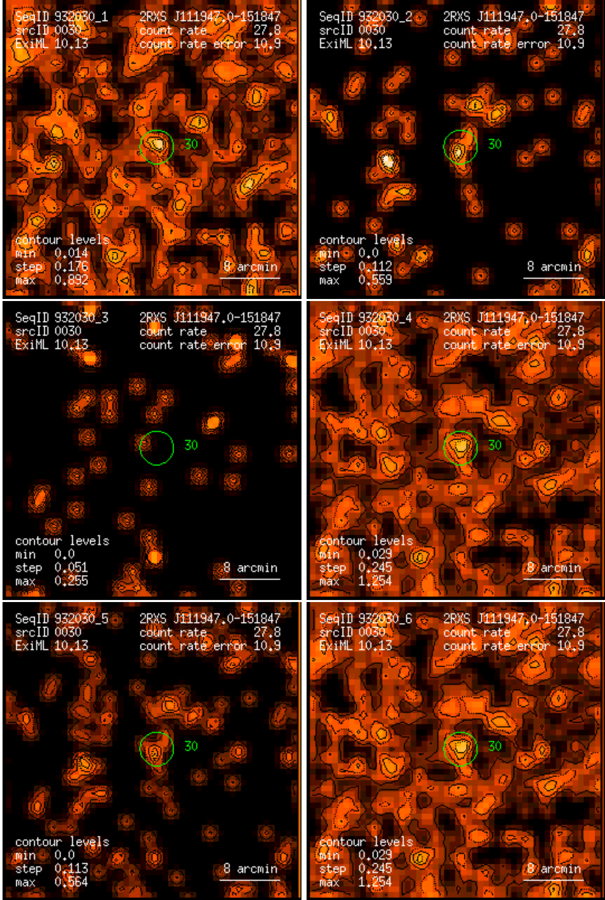
Figure 30: RASS 932030: detection 0030: band rate images, Gaussian filter: (1) PSPC channels 11 – 41, (2) 52 – 90, (3) 91 – 201, (4) 11 – 235, (5) 52 – 201, (6) 11 – 201. Broad band rates in counts/ks. Band rate contour levels in counts/ks/arcmin 2 .
