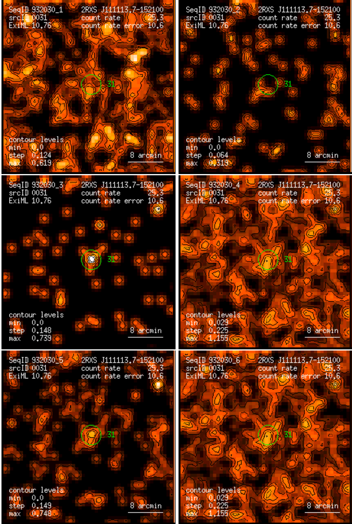
Figure 31: RASS 932030: detection 0031: band rate images, Gaussian filter: (1) PSPC channels 11 – 41, (2) 52 – 90, (3) 91 – 201, (4) 11 – 235, (5) 52 – 201, (6) 11 – 201. Broad band rates in counts/ks. Band rate contour levels in counts/ks/arcmin 2 .
